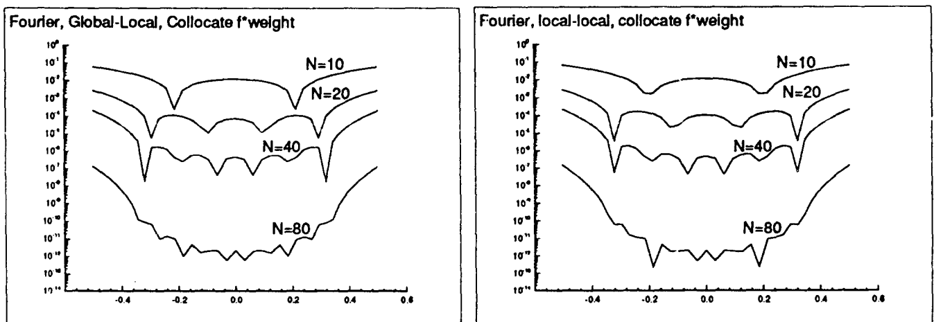
Fig. 1: Errors in log scale, f(x) defined by (5.1). [a, b] = [-0.5, 0.5] . Fourier collocation with Procedure A , namely interpolating f(x) * \alpha(x) with \alpha(x) defined by (3.7). \lambda = 0.4\epsilon N and m = 0.2\epsilon N , N = 10, 20, 40, 80 . Left: global-local ; Right: local-local .
