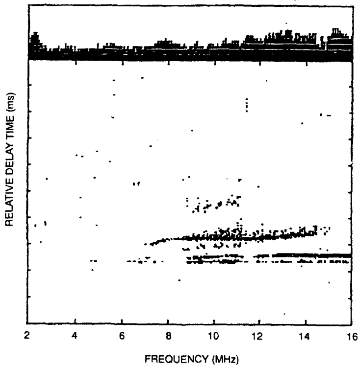
(b) Plot taken at 12:00:15 PST on 1 January 1994.
