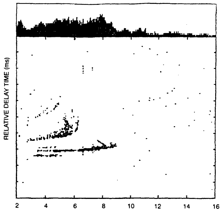
(a) Plot taken at 00:20:15 PST on 1 January 1994.
