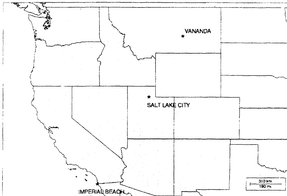
Figure 1. Relative locations of the transmitter site (Vananda), receiver site (Imperial Beach), and approximate path mid-point (Salt Lake City).
