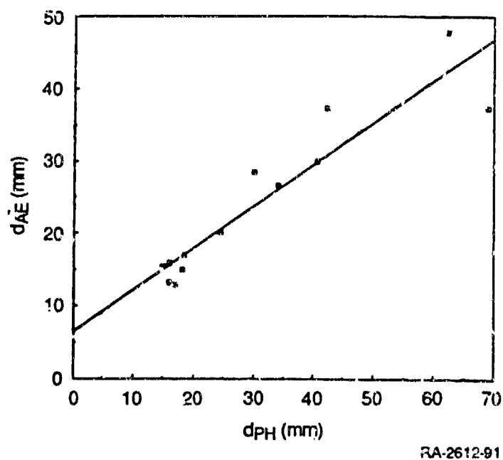
Figure B-9. Plot of dAE versus dPH .
