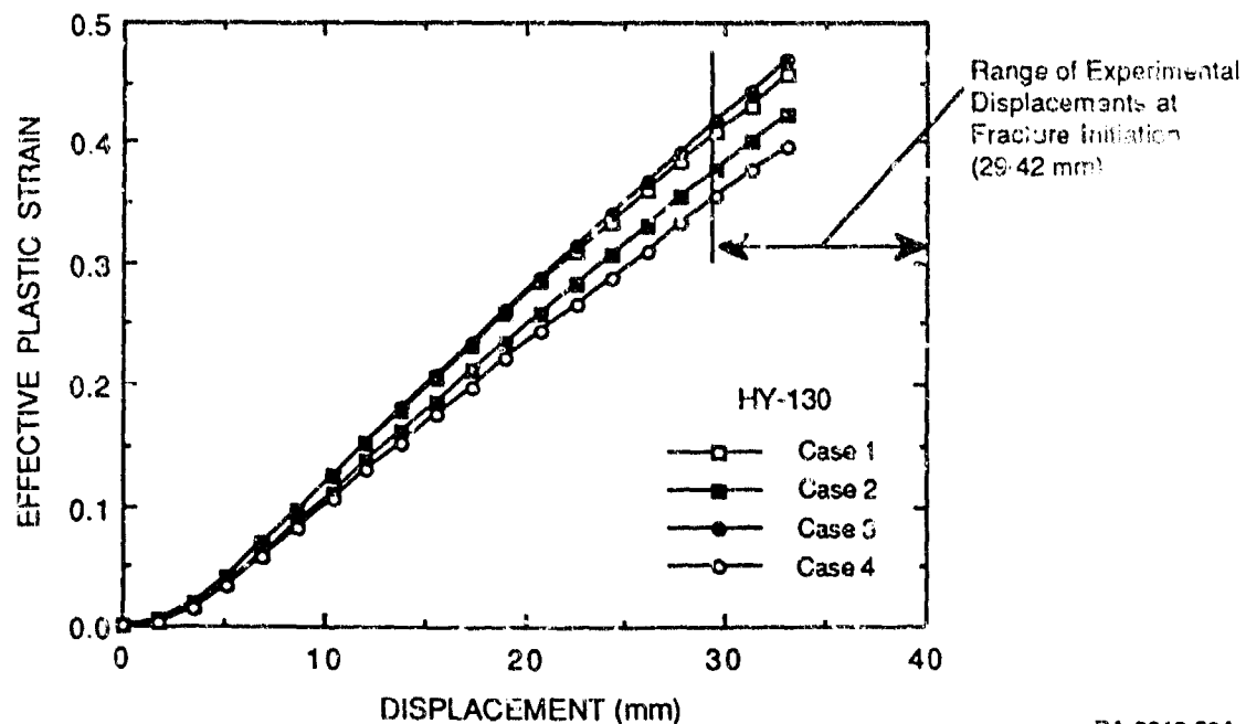
Figure D-9. Effective plastic strain as a function of specimen displacement for base plate HAZ element immediately at the toe of the weld bead for Cases 1 through 4.
