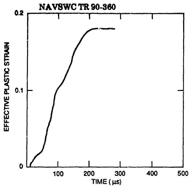
(a) V_0 = 110 m/s
