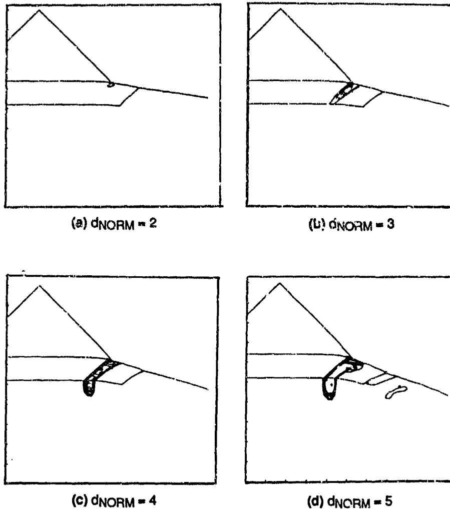
Figure D-19. Contours of damage in a simulated 1/4-scale static fracture experiment, showing a crack extending through HAZ and into the specimen plate
