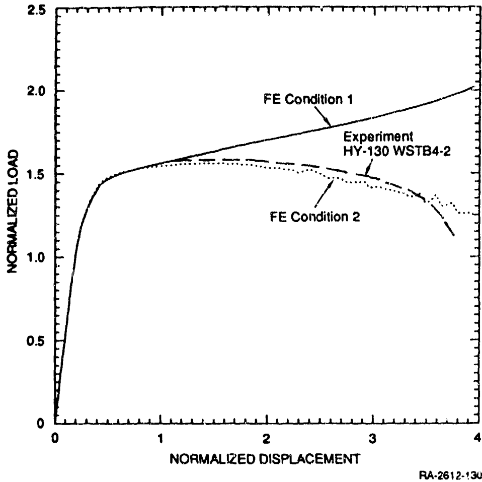
Figure D-18. Comparison of the normalized load-deflection curves for the finite element simulations with conditions 1 and 2 and with results of experiment HY-130 WSTB4-2.
