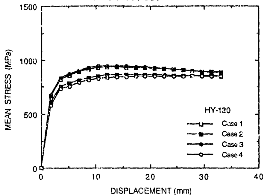
Figure D-8. Mean stress as a function of specimen displacement for base plate HAZ element immediately at the toe of the weld bead for Cases 1 through 4.
