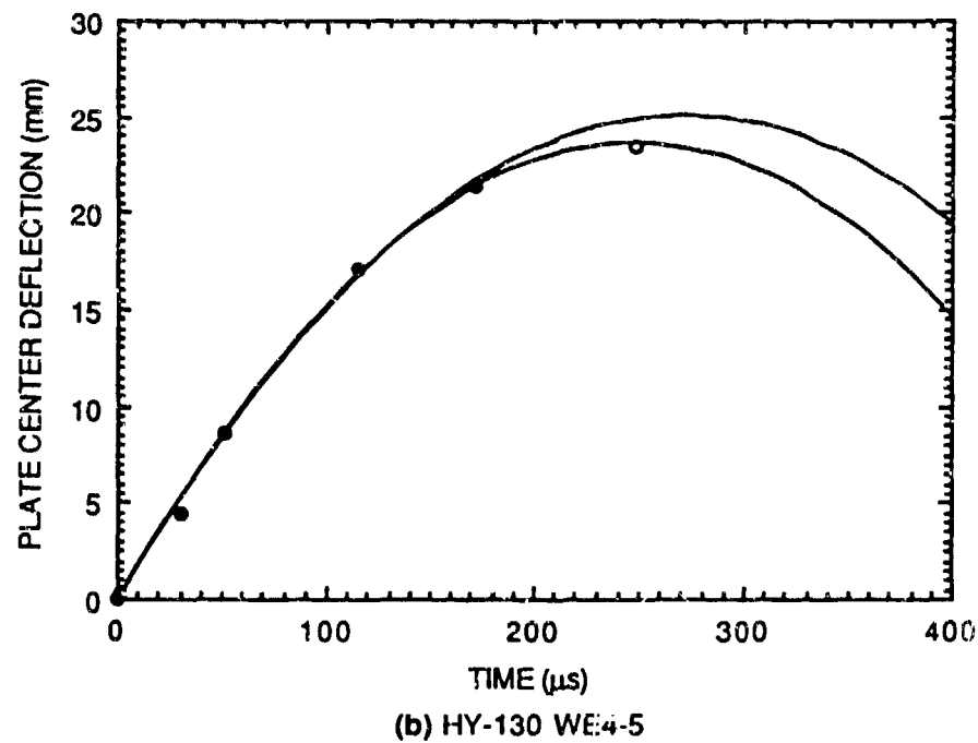
Figure C-18. Plate center deflection histories for experiments HY-130 WE4-4 and -5.
