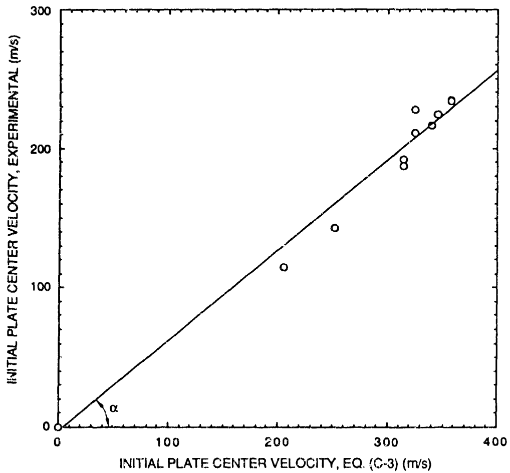
Figure C-28. Estimation of parameter \alpha from the predicted and measured values of V_0 .
