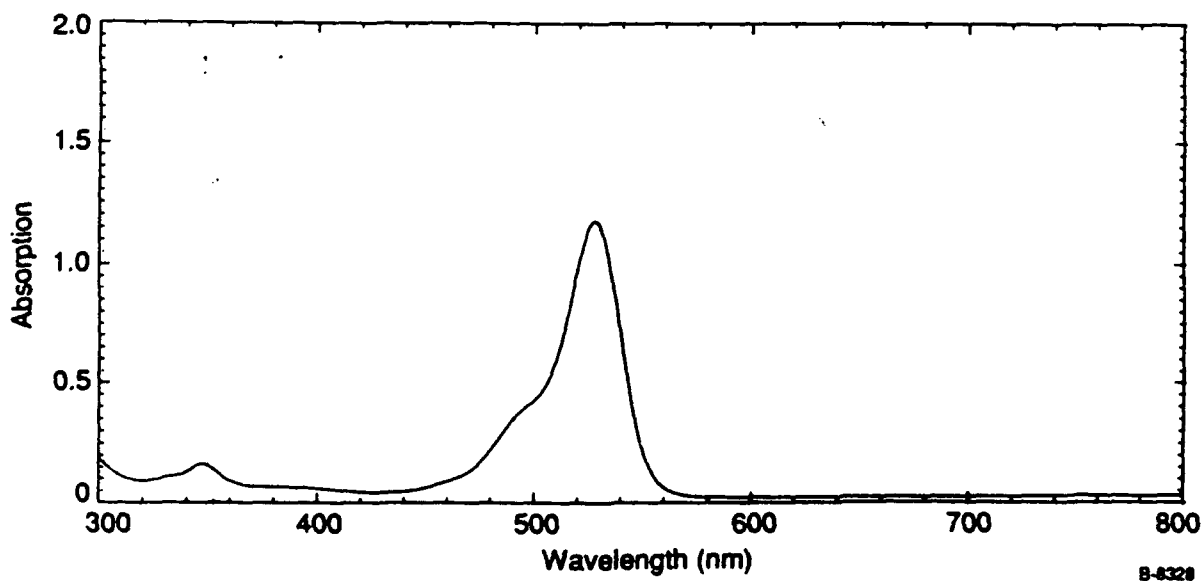
Figure 2. Absorption Spectrum for Rd-590 Dye at a Concentration of 1.23 \times 10^{-5}M
