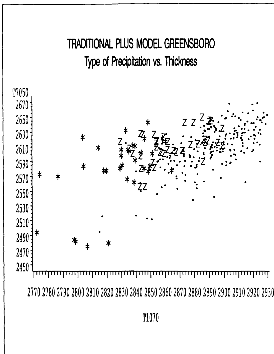
Figure 2.3. Nomogram of main precipitation type based on the Traditional Plus model for Greensboro, NC. T1070 along the X-axis is the 1000-700mb thickness in meters. T7050 along the Y-axis is the 700-500mb thickness in meters. Type is plotted as follows: * indicates frozen precipitation; Z indicates freezing precipitation; and • indicates liquid precipitation.
