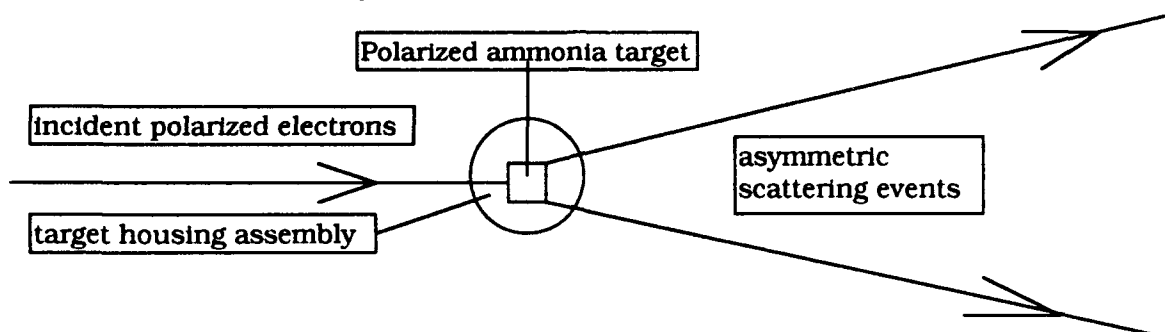
Figure 1. E143 experiment schematic
