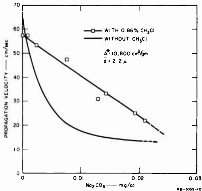
FIG. 13 STOICHIOMETRIC CH 4 -AIR — THE EFFECT OF CH 3 Cl ON THE EFFECTIVENESS OF Na 2 CO 3
