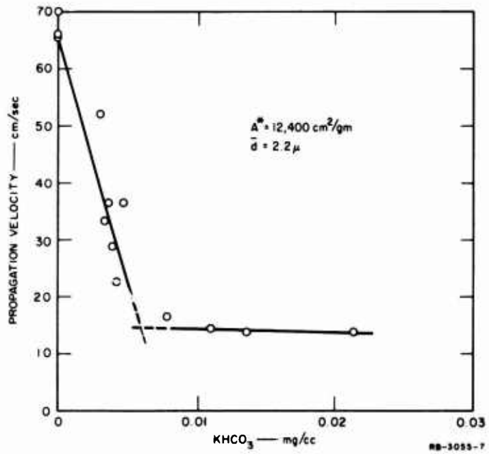
FIG. 9 STOICHIOMETRIC CH 4 -AIR—EFFECT OF KHCO 3 ON PROPAGATION VELOCITY
