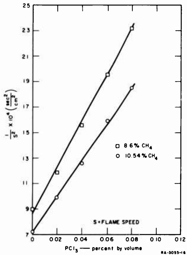
FIG. 4 \text{CH}_4 -AIR — 1/S^2 VERSUS CONCENTRATION OF \text{PCl}_3
