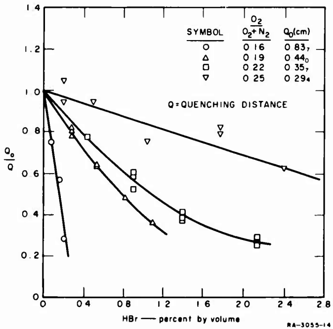
FIG. 2 CH_4-O_2-N_2-O_2 CONCENTRATION VERSUS QUENCHING EFFECTIVENESS OF HBr
