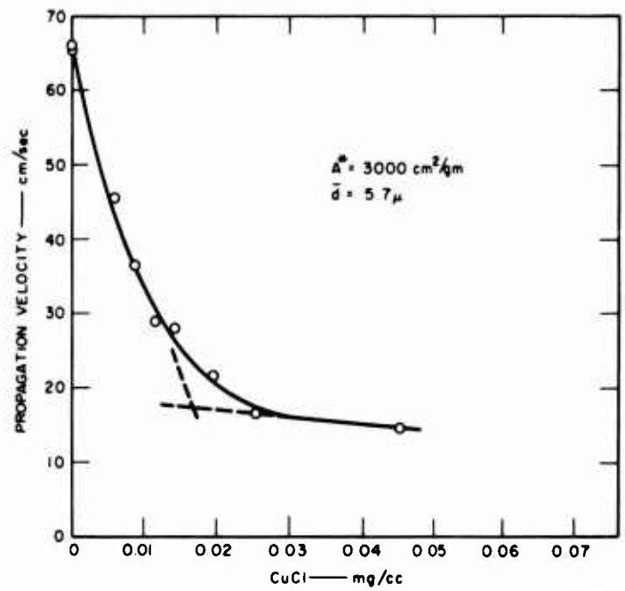
FIG. 11 STOICHIOMETRIC CH 4 -AIR—EFFECT OF CuCl ON PROPAGATION VELOCITY
