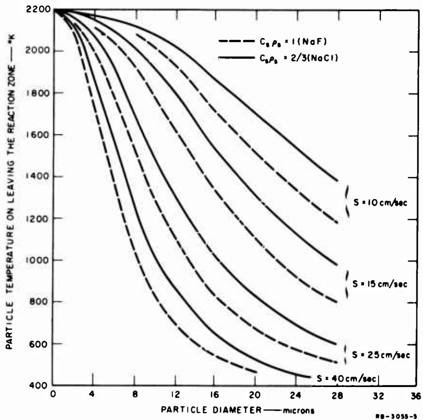
FIG. 15 THE TEMPERATURE REACHED BY SMALL NONEVAPORATING PARTICLES DURING PASSAGE THROUGH A STOICHIOMETRIC CH_4 -AIR FLAME
