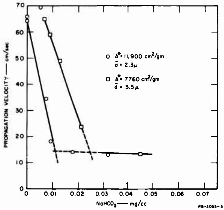
FIG. 8 STOICHIOMETRIC CH 4 -AIR — EFFECT OF NaHCO 3 ON PROPAGATION VELOCITY
