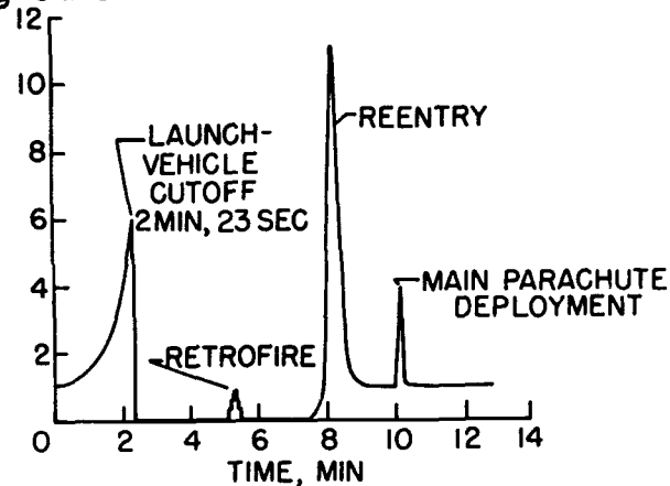
FIGURE 2-6. Acceleration time history for MR-4 flight.
