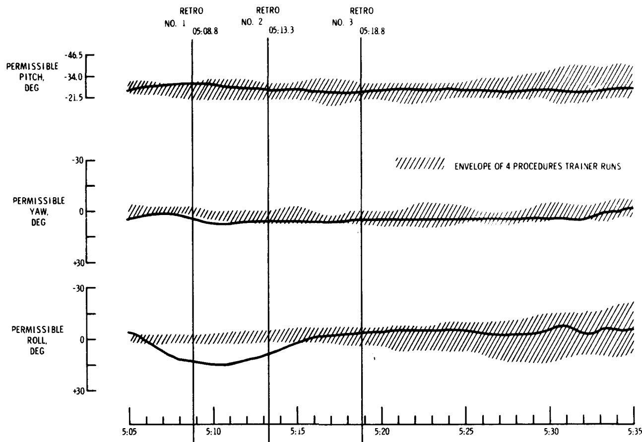
FIGURE 6-3. Attitude control during MR-4 retrofire period.
