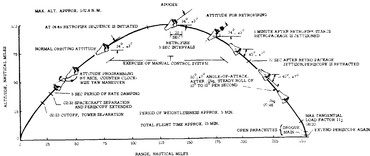
FIGURE 2-5. Flight profile for MR-4.
