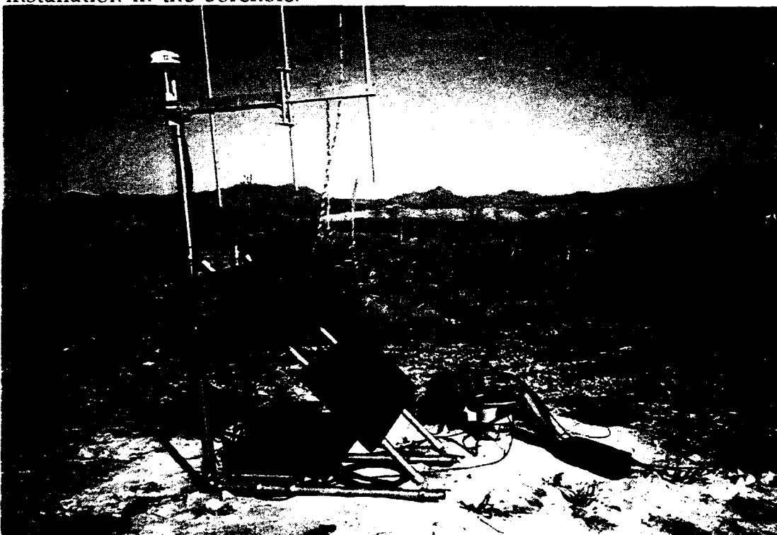
Figure 1b. Photograph of a prototype solar power array and antenna mounting being tested at the LTX station.
