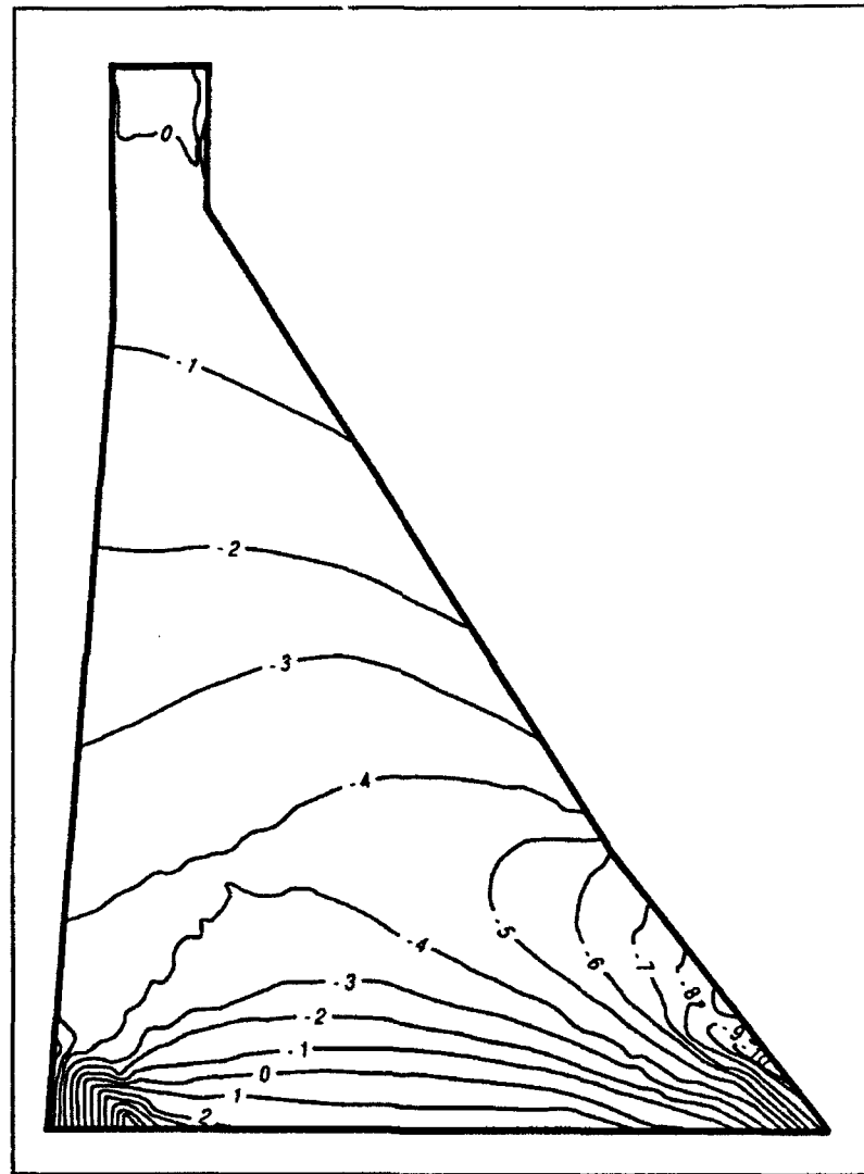
Figure 39. E_r/E_c = 0.05 , horizontal stress contours
