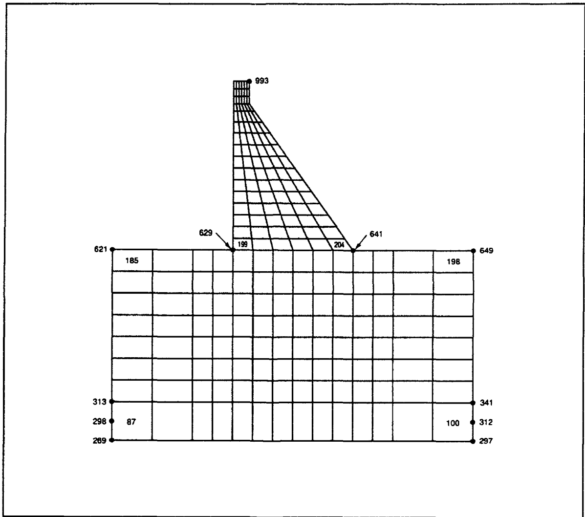
Figure 26. Mode' 1 (1.5-BW x 3-BW foundation model)
