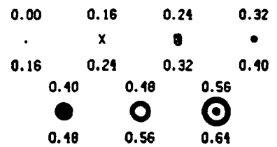
Figures 13a.-13b. Marginal Probability of Dry El Viejo Years during (a) OND and (b) NDJ for Seasonal Mean Monthly Precipitation. The key to probabilities is at right.
