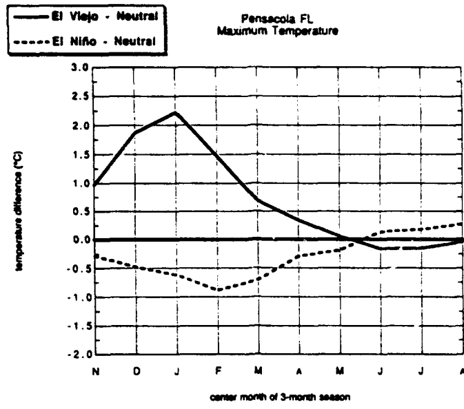
Figure 5g. Difference in ENSO Category Means during the ENSO Year for Seasonal Mean Maximum Temperature at Pensacola FL. Same as in Figure 5a.
