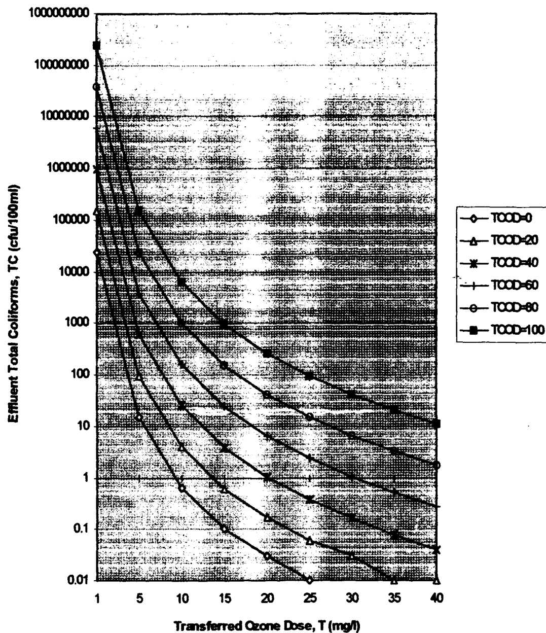
Figure 19. Ozone Disinfection Efficiency with Respect to TOOD and the Transferred Ozone Dose.
