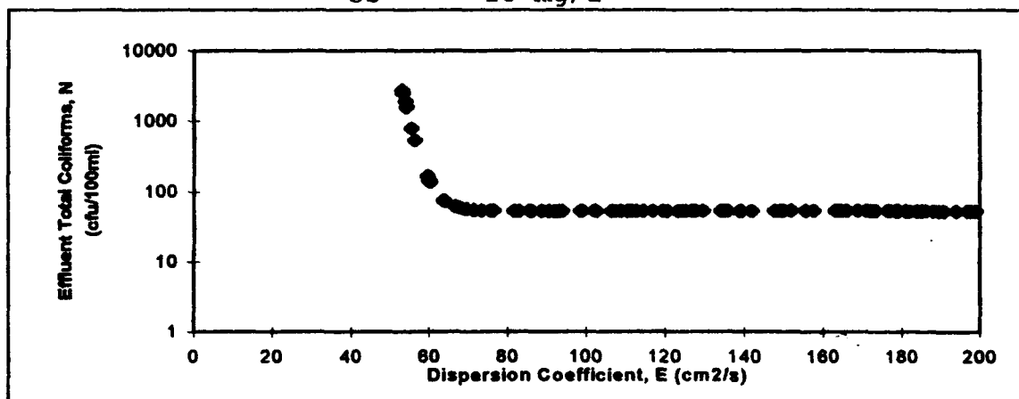
Figure 14. Effect of Varying Dispersion Coefficient, E.
