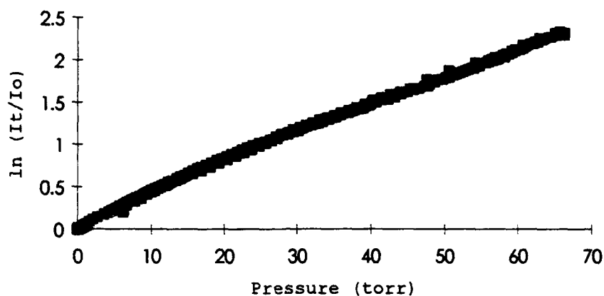
Figure 13. Corrected Cross-Sectional Area Plot
