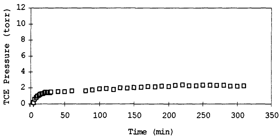
Figure 15. Desorption of TCE from Flint Clay
