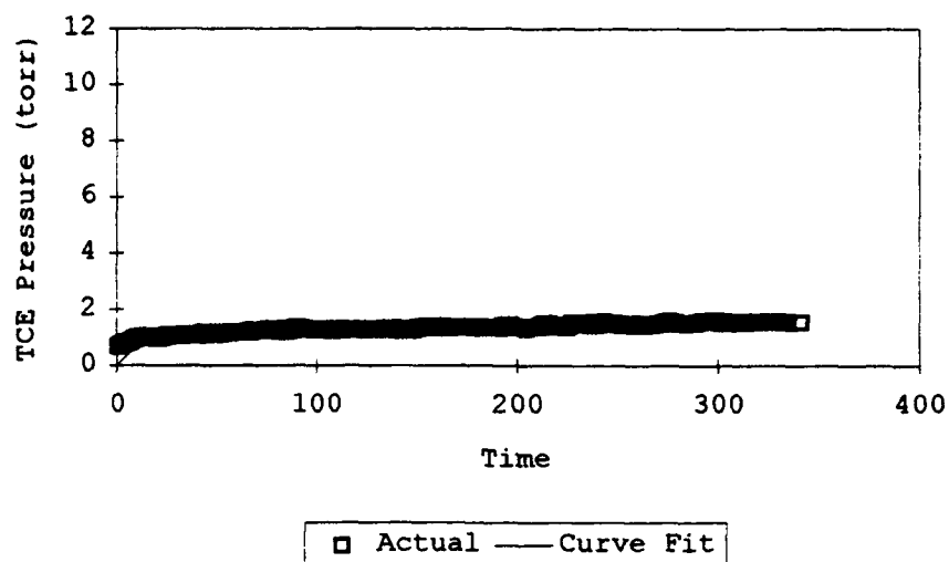
Figure 27. Curve Fit of Langmuir Isotherm Functional Form to TCE Desorption from Sodium Feldspar Data.
