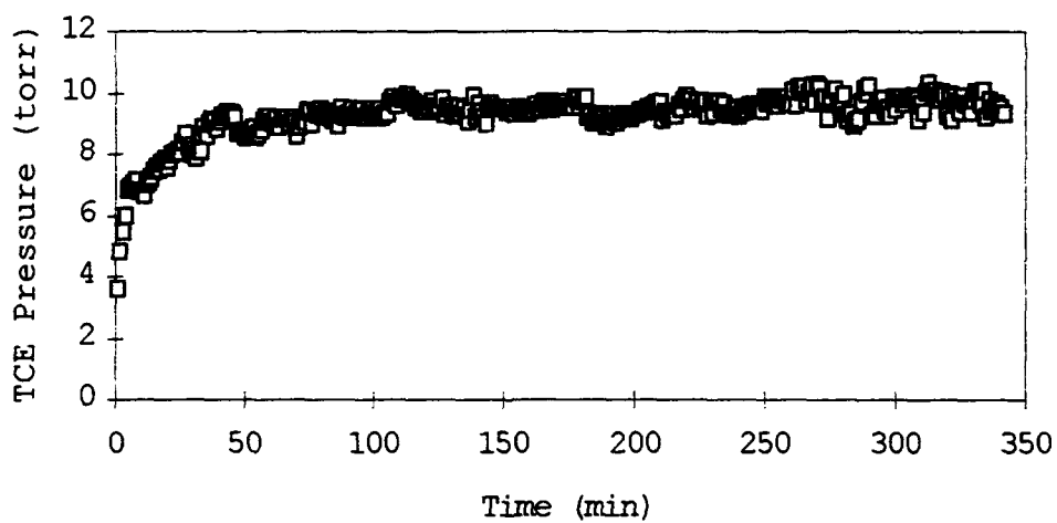
Figure 17. Desorption of TCE from Montana Soil
