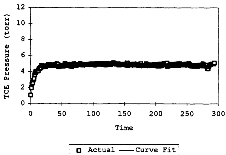
Figure 21. Curve Fit of Langmuir Isotherm Functional Form to TCE Desorption from Dolomitic Limestone Data.
