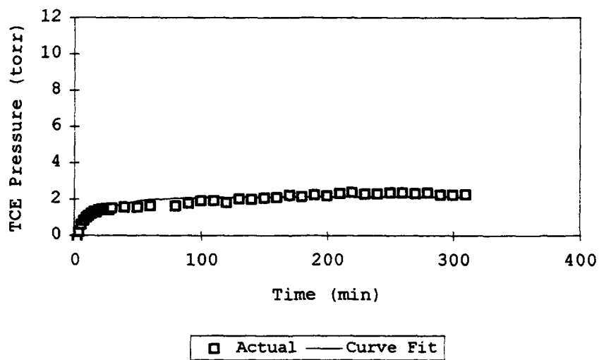
Figure 22. Curve Fit of Langmuir Isotherm Functional Form to TCE Desorption from Flint Clay Data.
