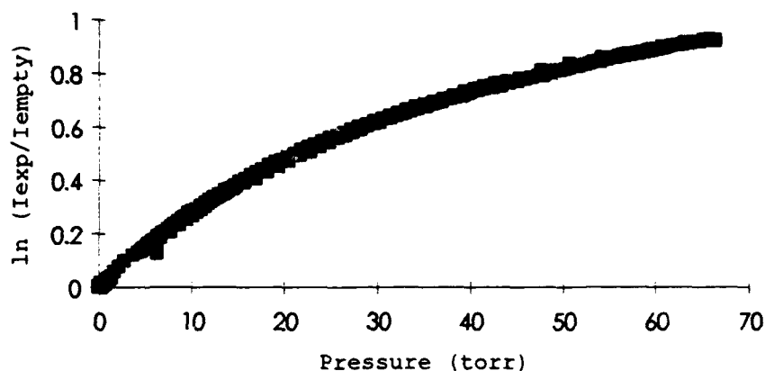
Figure 9. Uncorrected Cross-Sectional Area Plot
