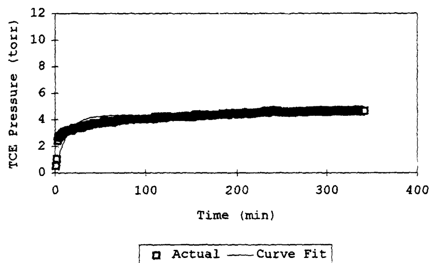
Figure 26. Curve Fit of Langmuir Isotherm Functional Form to TCE Desorption from San Joaquin Soil Data.
