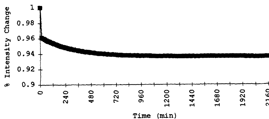
Figure 5. Curve Fit of Detector 2 Drift.
