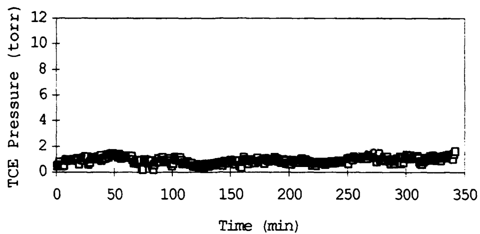
Figure 16. Desorption of TCE from Glass Sand
