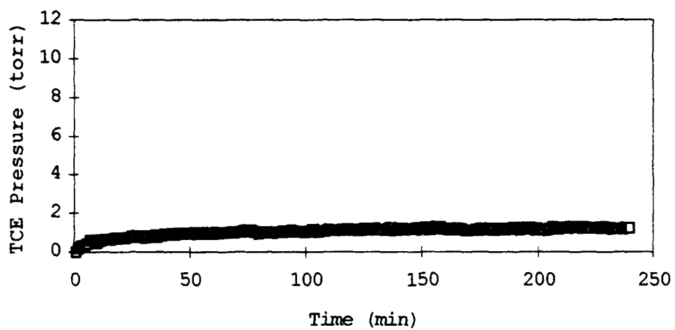
Figure 18. Desorption of TCE from Plastic Clay
