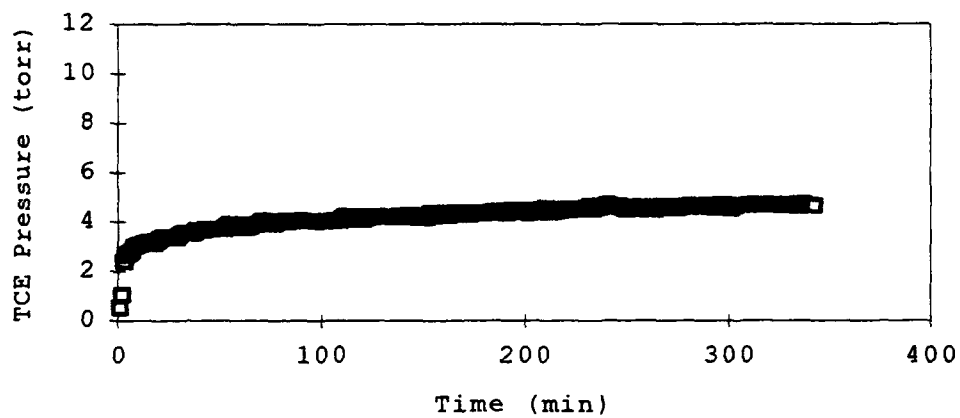
Figure 19. Desorption of TCE from San Joaquin Soil
