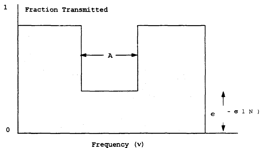
Figure 10. Rectangular Approximation of TCE Transmission
