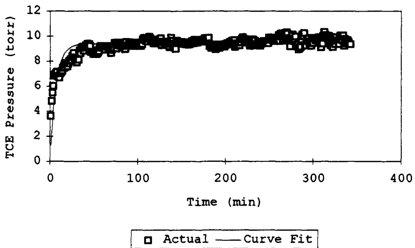
Figure 24. Curve Fit of Langmuir Isotherm Functional Form to TCE Desorption from Montana Soil Data.
