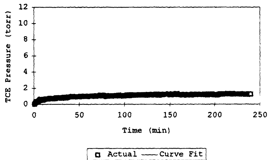
Figure 25. Curve Fit of Langmuir Isotherm Functional Form to TCE Desorption from Plastic Clay Data.
