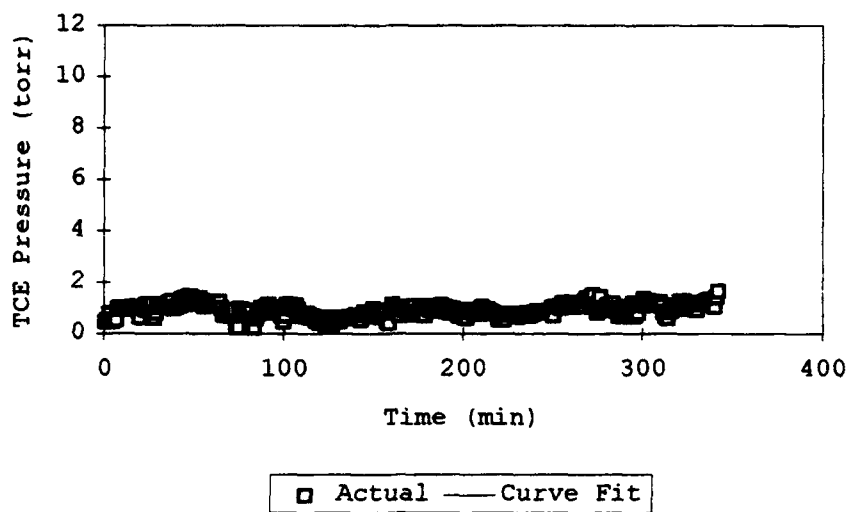
Figure 23. Curve Fit of Langmuir Isotherm Functional Form to TCE Desorption from Glass Sand Data.
