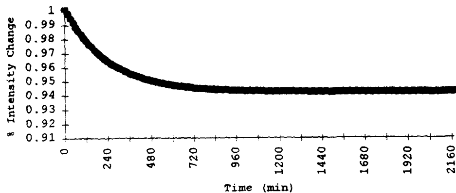
Figure 4. Curve Fit of Detector 1 Drift.
