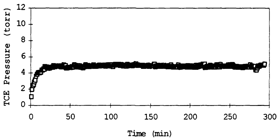
Figure 14. Desorption of TCE from Dolomitic Limestone
