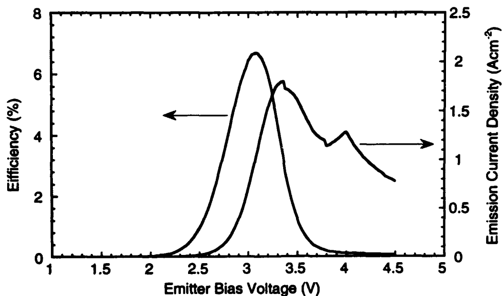
FIG. 15 Emission characteristics of a AlGaAs/GaAs PDBEE with the channel layer within the emission areas partially removed.
