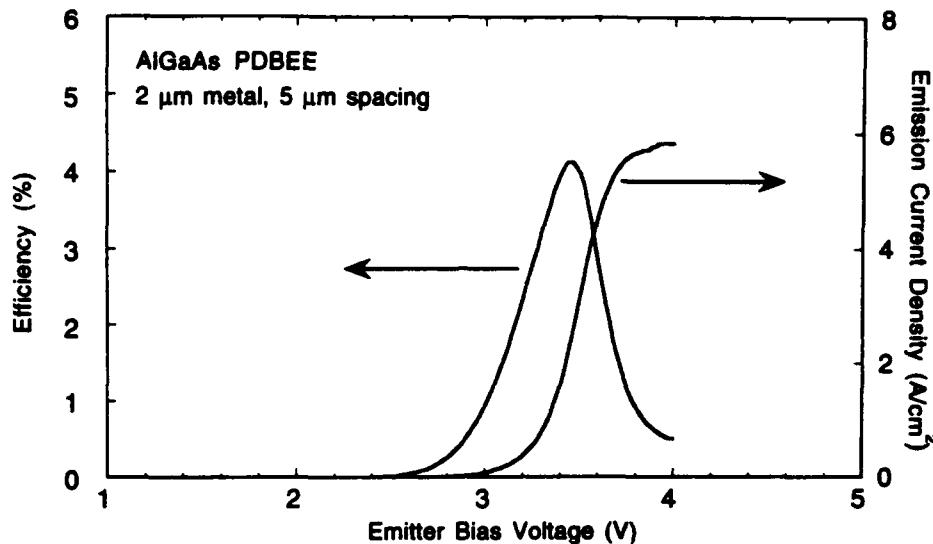
FIG. 13 Emission characteristics of a \text{AlGaAs}/\text{GaAs} PDBEE.
