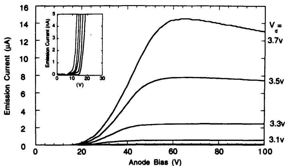
FIG. 14 Emission current vs. anode voltage at different emitter bias voltages as indicated in the figure. The anode bias is scanned from zero to 100 voltages. The insert is the blow-up at low current levels.
