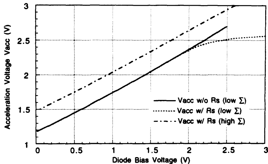
FIG. 4 Calculated acceleration voltage as a function of the bias voltage for two PDB diodes. The solid line is for the PDB diode shown in Fig. 2.7 which has a lower p+ delta doping density ( \Sigma ) without taking the series resistance into account, the dashed line is for the same diode with a series resistance, and dot-dashed line is for the diode with a higher \Sigma and a series resistance.
