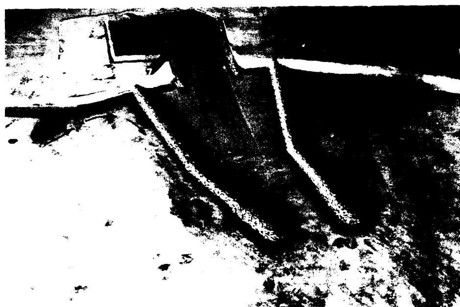
Photo 52. General movement of tracer material and subsequent deposits for Plan 3; 7-sec, 10-ft waves from the northwest; swl = +4.4 ft
