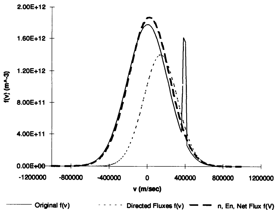
Figure 27. Comparison of Distribution Function Based on Directed Flux Matching to Our Implementation.
