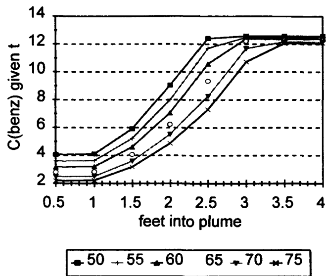
Figure A2-1. C(\text{benz}) over Plume Length. @ t = 50 to 75 days.
