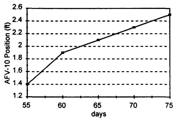
Figure A2-12. AFront Position over time to 75 days with data: BTEX = 33, V_{\text{rel}} = 1\text{ft/d} , O_2 = 4
