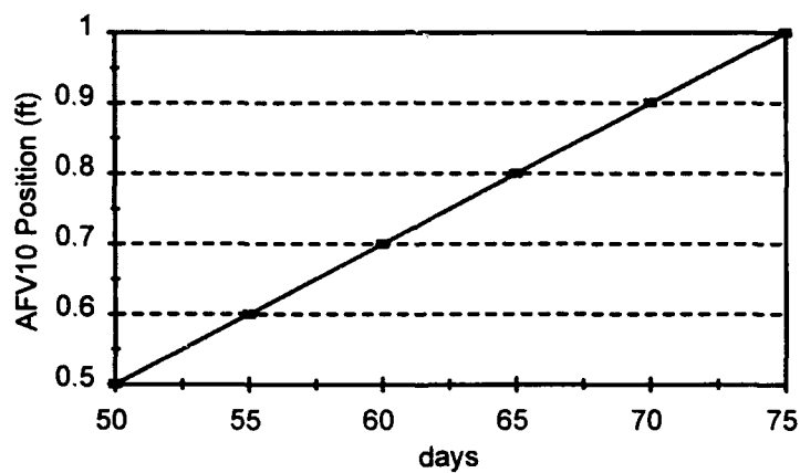
Figure A2-32. AFront Position over time to 75 days with data: O_2 = 3.5 , BTEX = 33 , V_{rel} = 0.5
