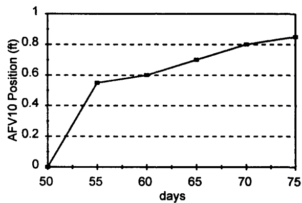
Figure A2-30. AFront Position over time to 75 days with data: O_2 = 3 , BTEX = 33, V_{\text{rel}} = 0.5
