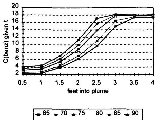
Figure A2-15 C(benz) over Plume Length, @ t = 50 to 75 days, with data: BTEX = 50, Vrel = 1ft/d, O2 =4
