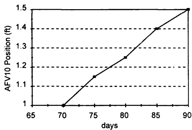
Figure A2-16. AFront Position over time to 75 days with data: BTEX = 50, Vrel = 1ft/d, O2 =4
