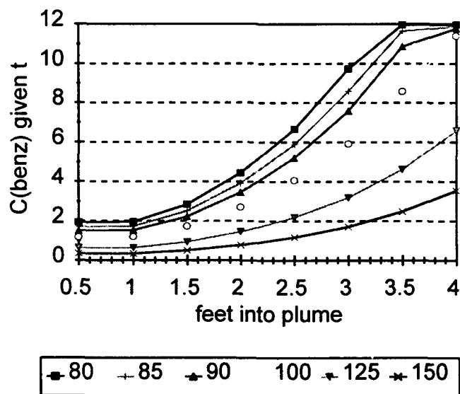
Figure A2-2. C(\text{benz}) over Plume Length. @ t = 75 days to 150 days.
