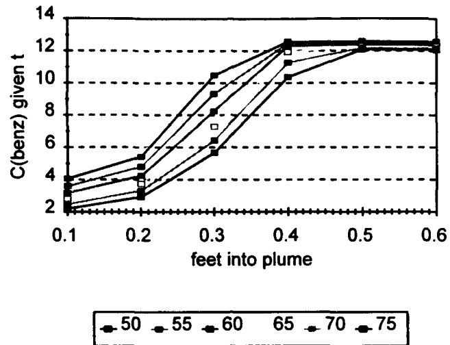
Figure A2-19 C(\text{benz}) over Plume Length, @ t = 50 to 75 days, with data: V_{\text{rel}} = 0.1 , BTEX = 33, O_2 = 4
