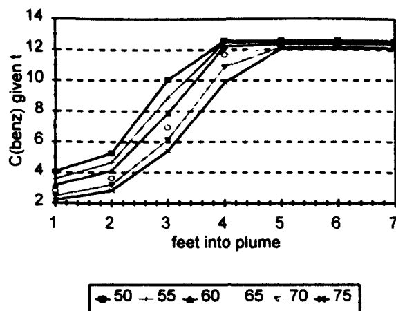
Figure A2-11 C(\text{benz}) over Plume Length, @ t = 50 to 75 days, with data: BTEX = 33, V_{\text{rel}} = 1\text{ft/d} , O_2 = 4
