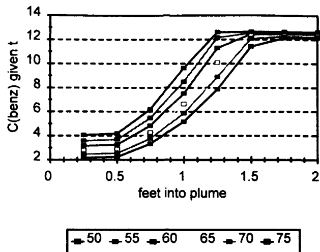
Figure A2-29 C(\text{benz}) over Plume Length, @ t = 50 to 75 days, with data: O_2 = 3 , BTEX = 33, V_{\text{rel}} = 0.5
