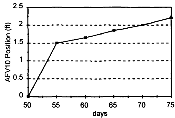
Figure A2-24. AFront Position over time to 75 days with data: V_{\text{rel}} = 1.0 , BTEX = 33, O_2 = 4
