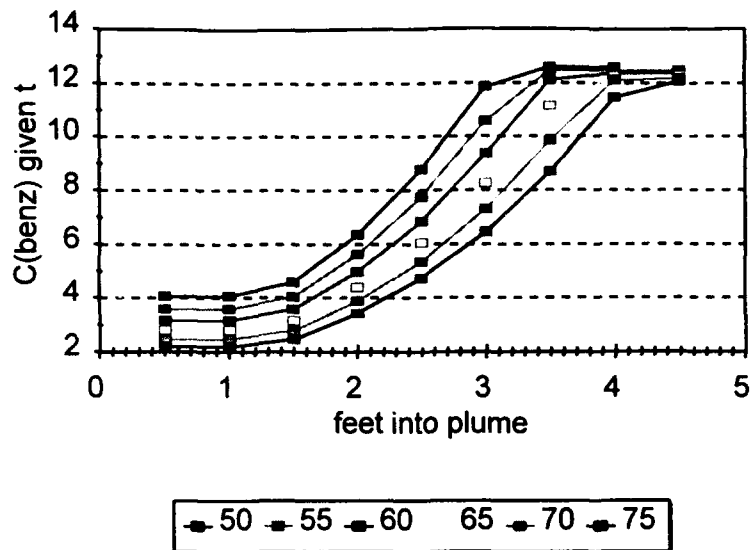
Figure A2-23 C(\text{benz}) over Plume Length, @ t = 50 to 75 days, with data: V_{\text{rel}} = 1.0 \text{ ft/d} , BTEX = 33, O_2 = 4
