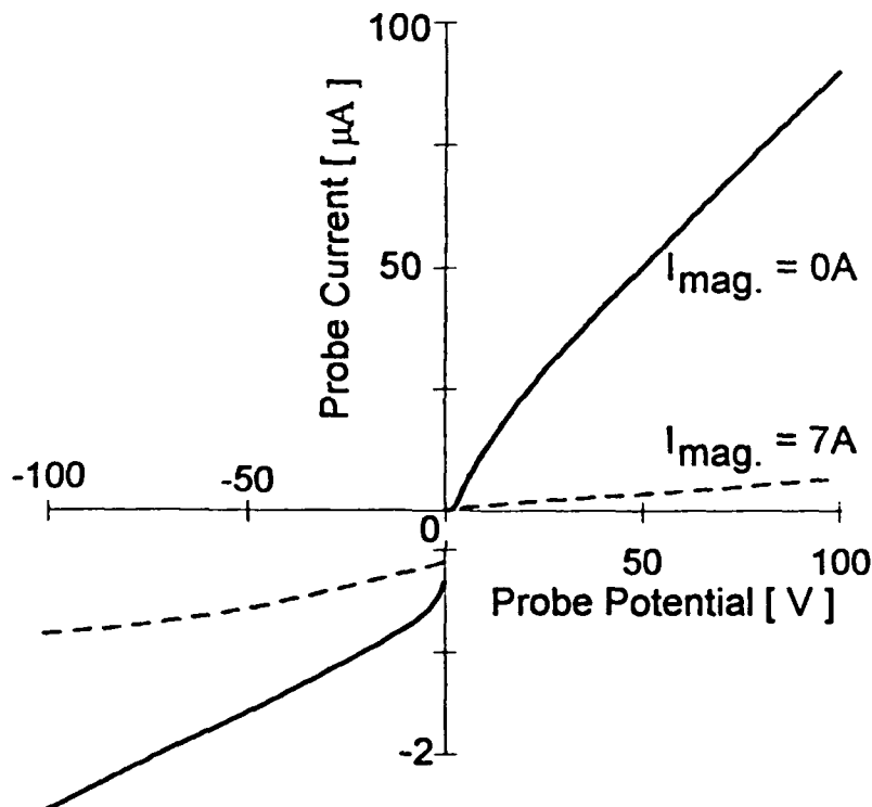
Figure 4 - I-V characteristics of Langmuir probe with the external solenoid current at 0A and 7A.
