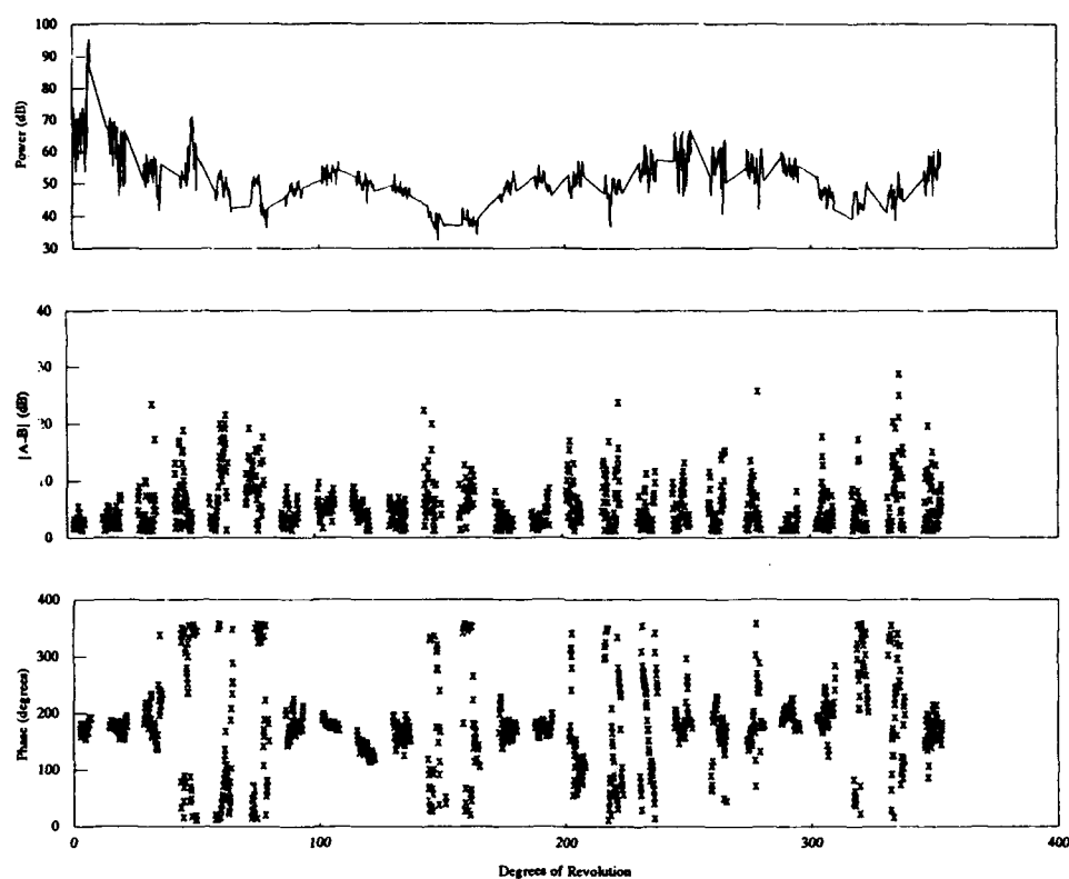
(c) FR8100 radar on Transporte : - 1st revolution of data file 8260804.dat in position 2
