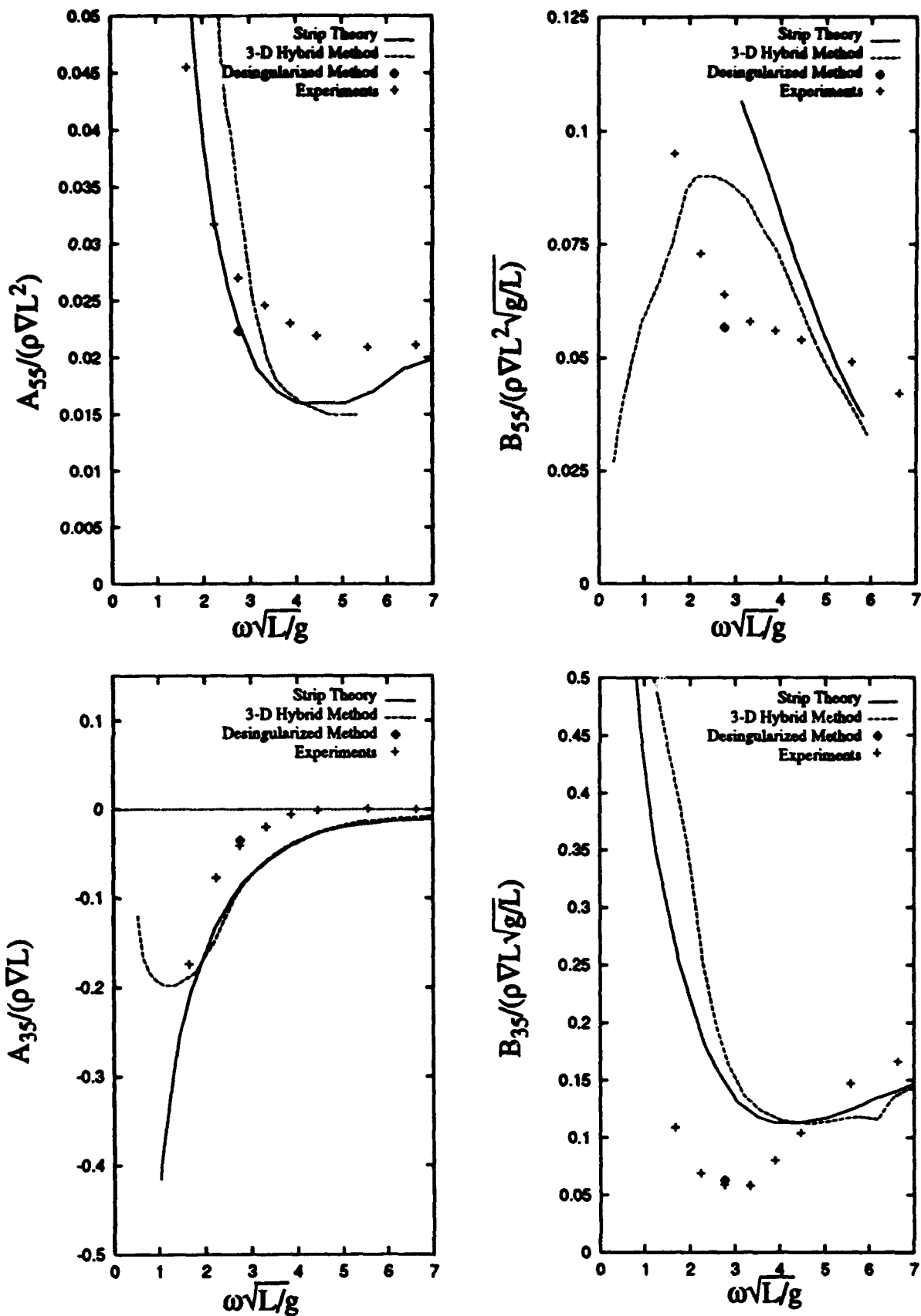
Comparisons of experimental and theoretical added mass and damping coefficients for forced pitch (Wigley model III, Fr = 0.3 , pitch amplitude = 1.5^\circ )
