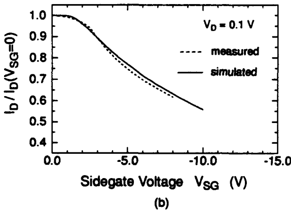
Figure 2. Measured and simulated sidegating effects due Gunn domain (a) and Schottky contact (b).
