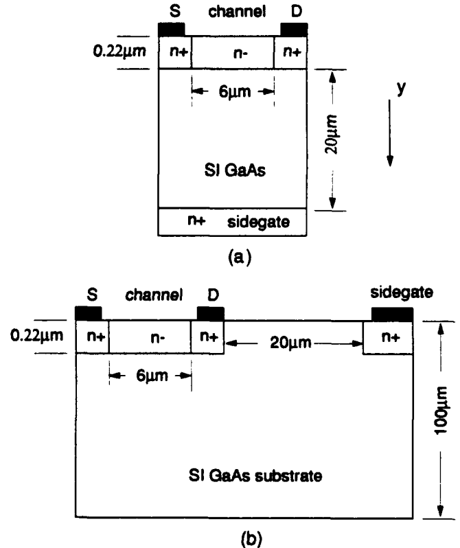
Figure 4. Vertical (a) and lateral (b) structures for simulations.
