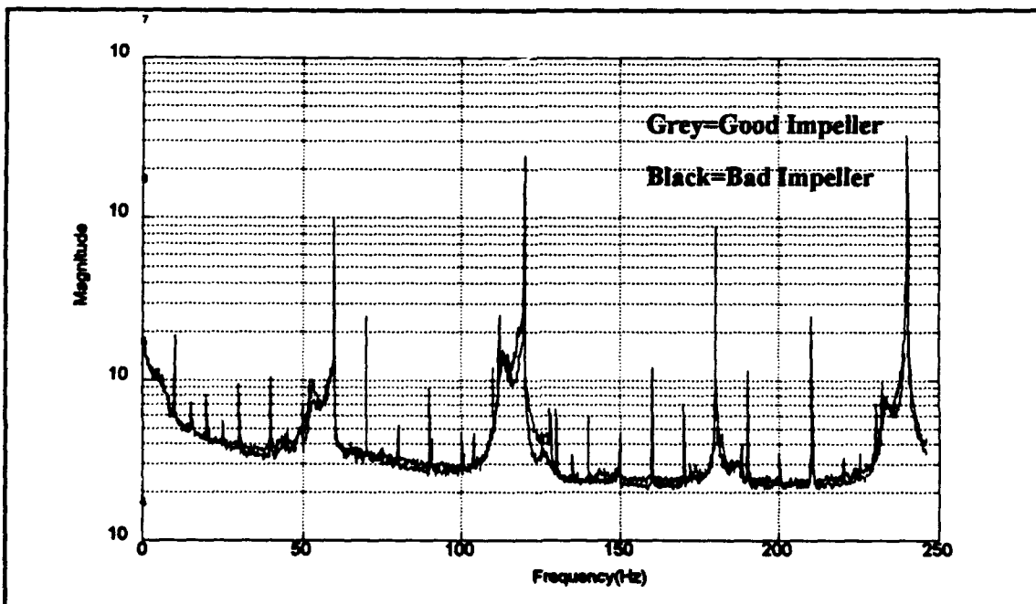
Figure 4.7 -The ensemble averaged AM demodulated spectra overlaid
