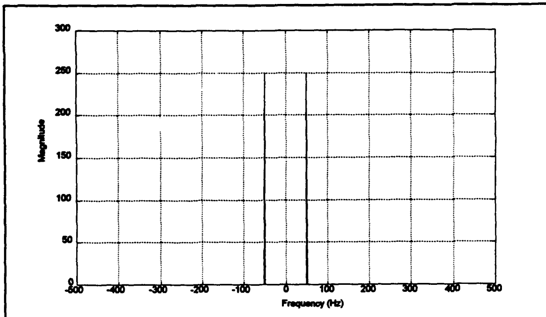
Figure 2.5-The magnitude spectrum of the AM demodulated signal
