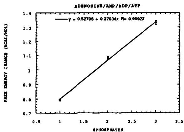
Figure 23. Changes in retention times (a.), and free energy (b.), per phosphate for the adenylate series.
