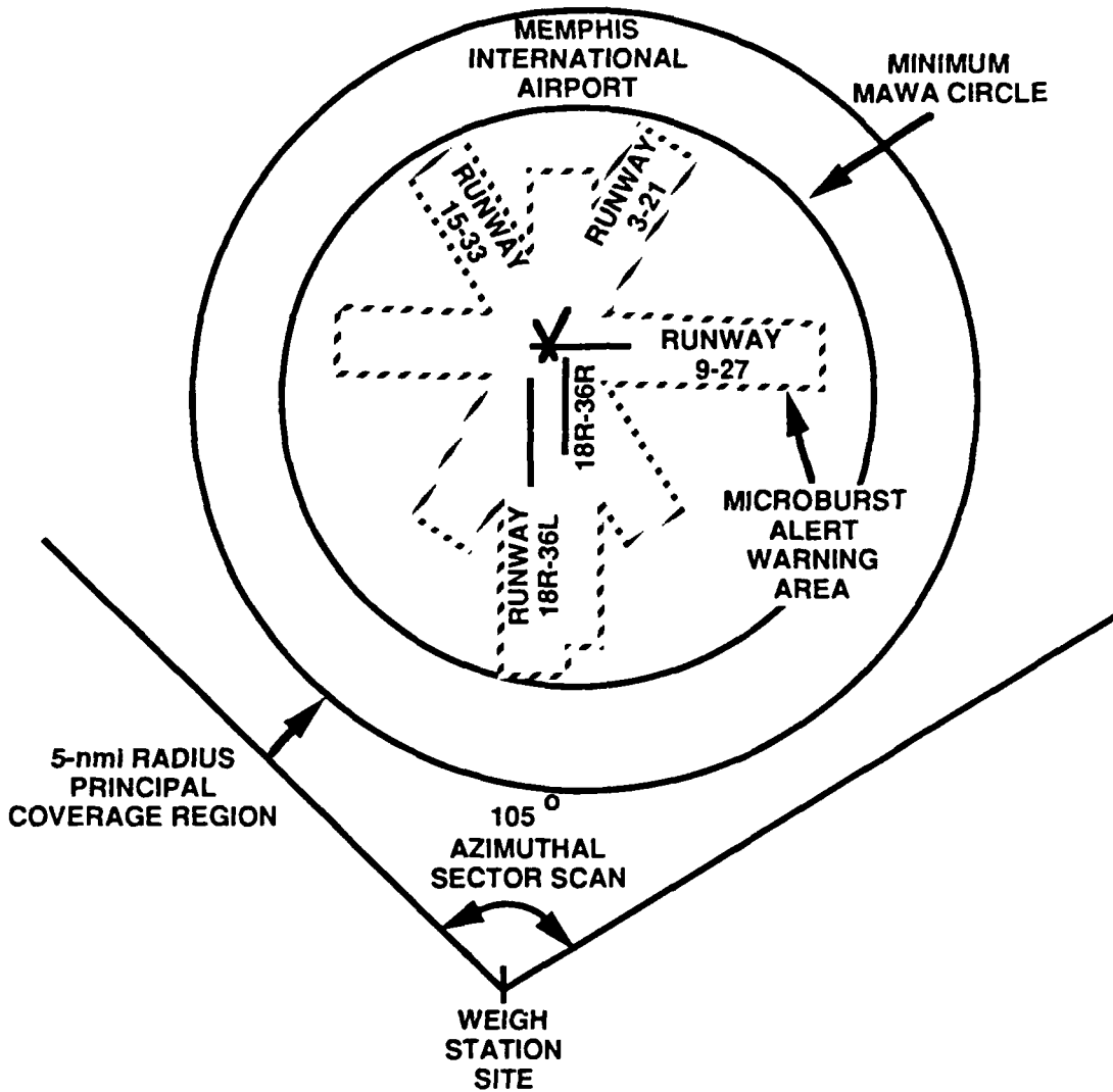
Figure 1. Azimuthal sector scan geometry for Memphis TDWR.
