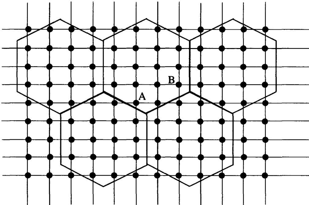
Figure 1: Hexagon partition in a 2d mesh
