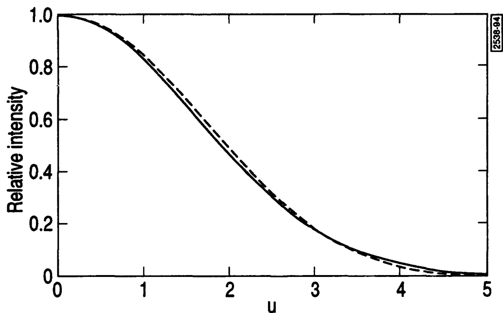
Figure 3. Far-field irradiance beam pattern of a truncated Gaussian beam as function of normalized angular coordinate u [= \theta/(\lambda/\pi D)] for d/D = 0.7 . The dashed and solid curves are based on the exact [i.e., Eq. (2.5)] and approximate [i.e., Eq. (2.9)] expressions for the beam pattern, respectively.
