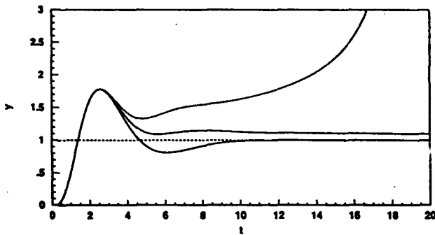
Figure 3: Sensitivity of certainty-equivalence based design using state- x for \theta = 1 , \hat{\theta} = 1 , 1.0025, 1.005.
