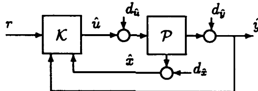
Figure 2.2: Feedforward system
