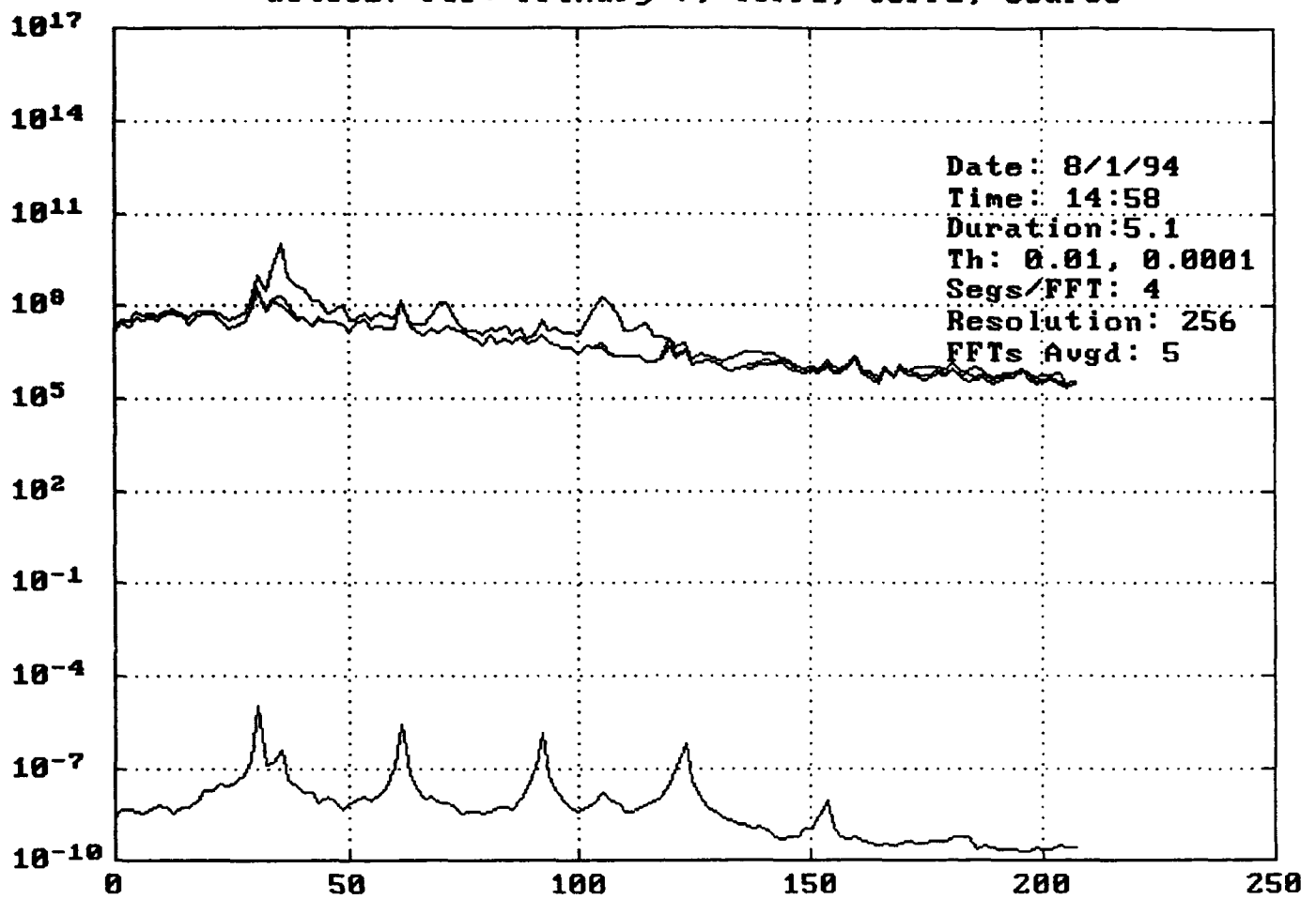
Figure VB-11. PSD's, Primary 7, corrected (2), source: 25 Hz sine wave
