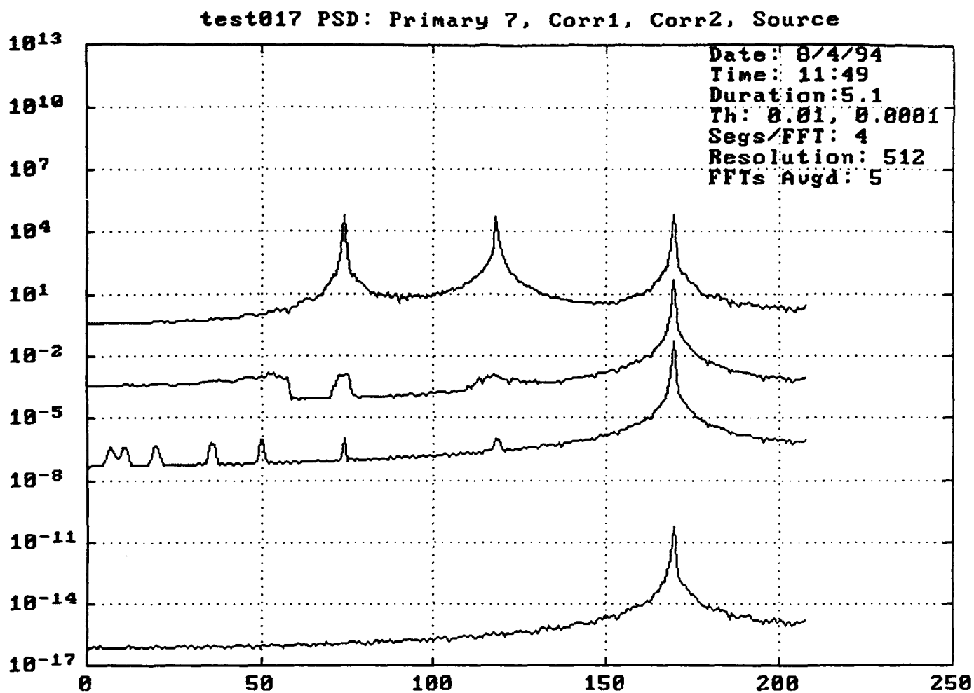
Figure VA-8. PSD's, Primary 7, corrected (2), source as in Fig. VA-4, but with 512 resolution: simulated test
