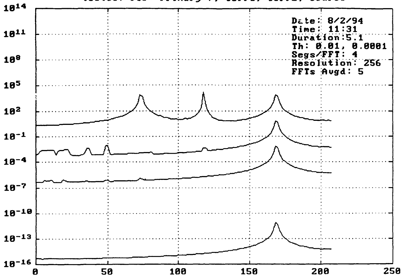
Figure VA-2. PSD's, Primary 7, corrected (2), source: simulated test
