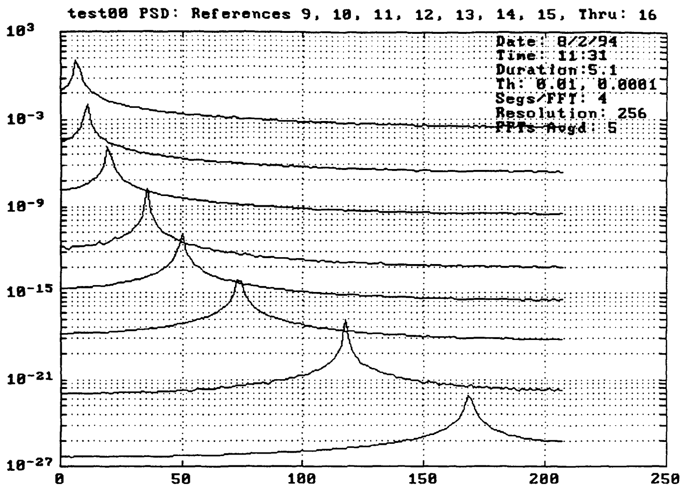
Figure VA-5. PSD's, References and source: simulated test
