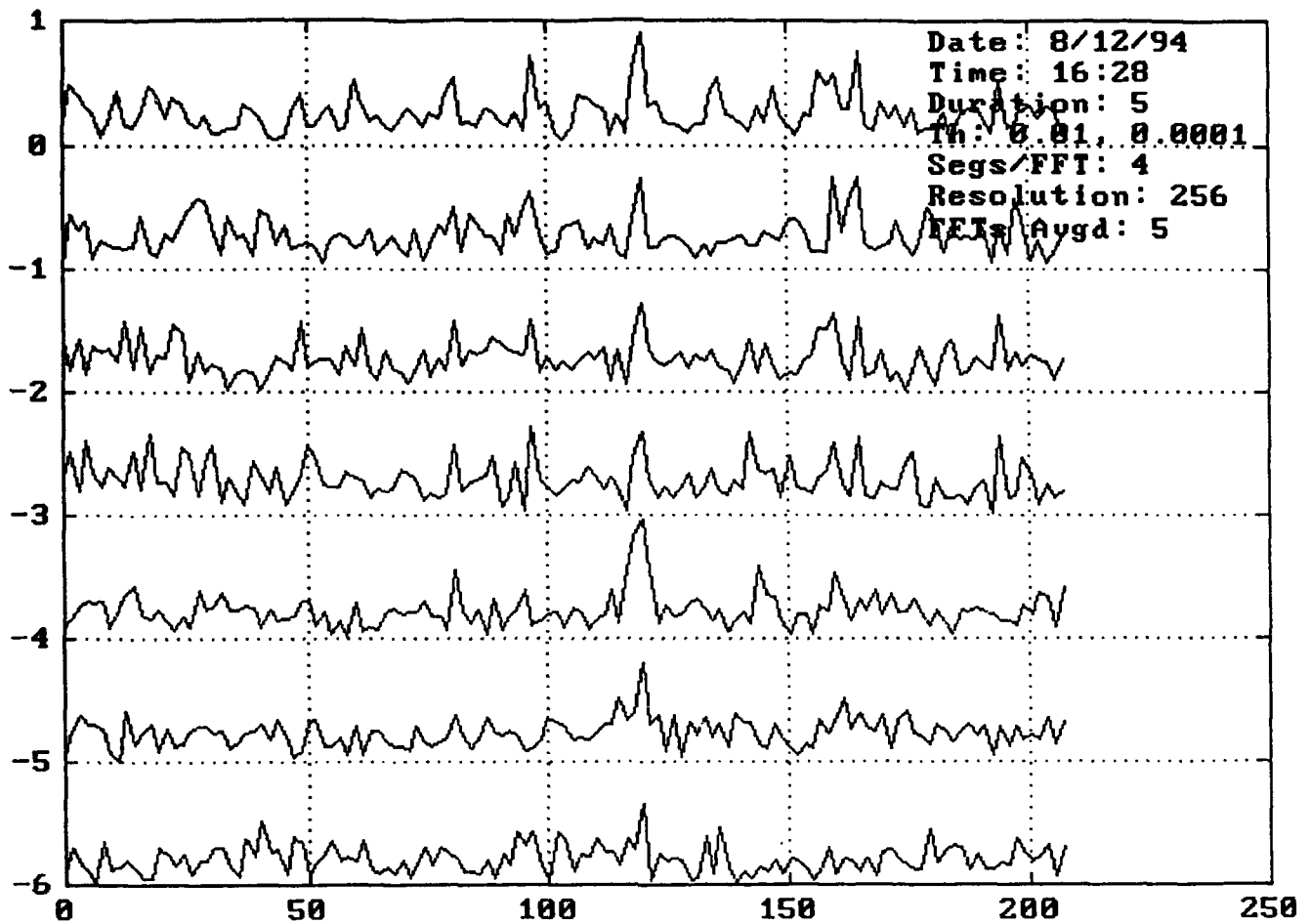
Figure VD-4. Lack of coherence at 80 Hz of all 7 references with Primary Microphone 1 explains failure in Fig. VD-2 to cancel peak at 80 Hz
