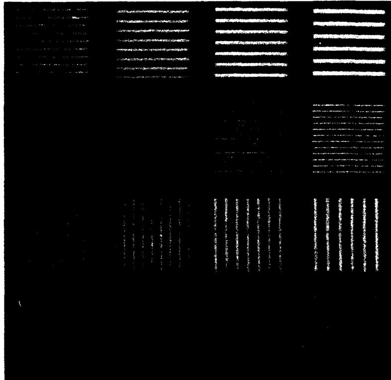
Figure 20. Bar pattern chart as seen by the full-aperture system. The system is just able to resolve the pattern in which the bar spacing is two pixels.
