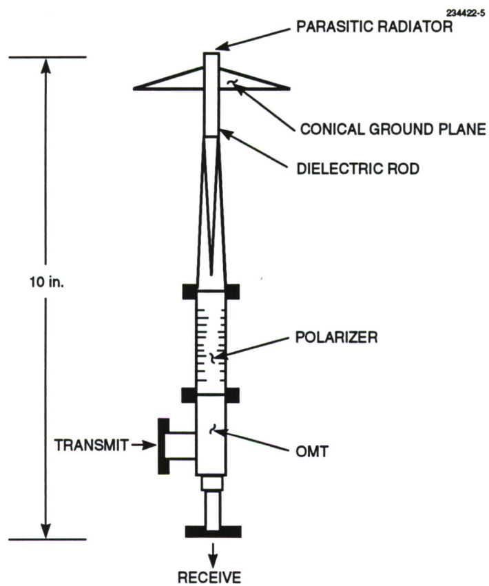
Figure 5. A K_u -band wide-beam antenna design.
