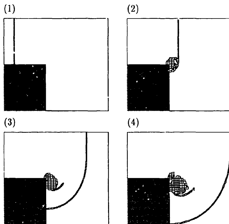
Figure 10: The AMR algorithm employs a dynamic grid system.
