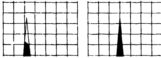
Figure 14: The tip of the knife edge with and without blunting.
