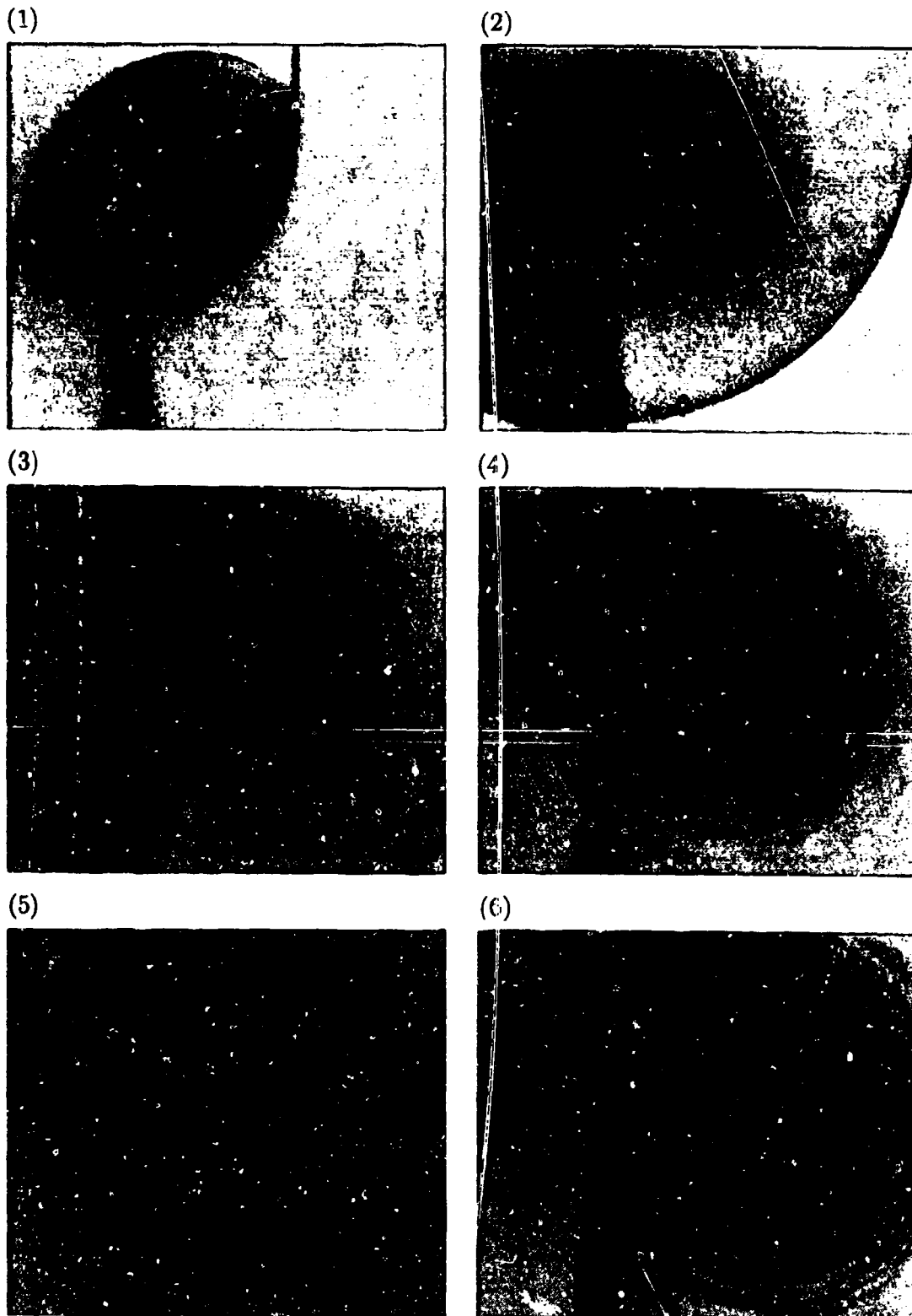
Figure 13: Evolution of a vortex sheet due to a shock wave diffracting over a knife edge.
