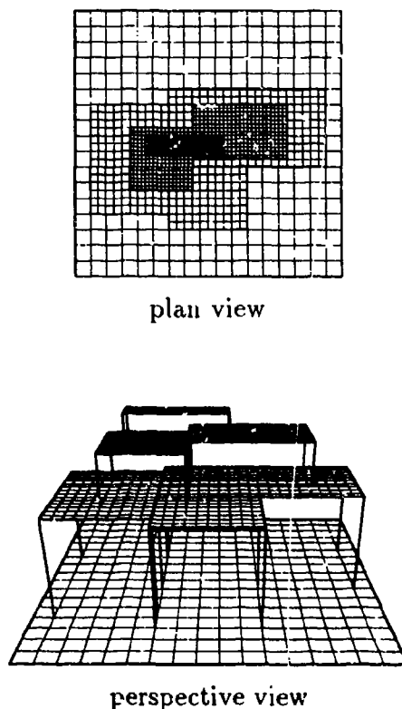
Figure 8: The AMR algorithm employs a hierarchical grid system.
