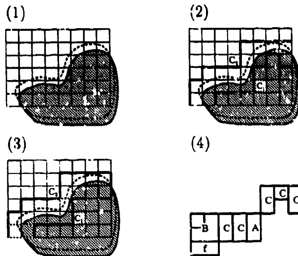
Figure 6: Strategy for finding groups of cells whose type remains constant when a body moves.
