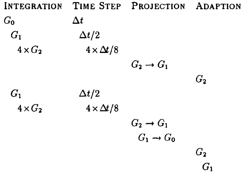
Figure 9: Grid operations are recursively interleaved (to be read from top to bottom).
