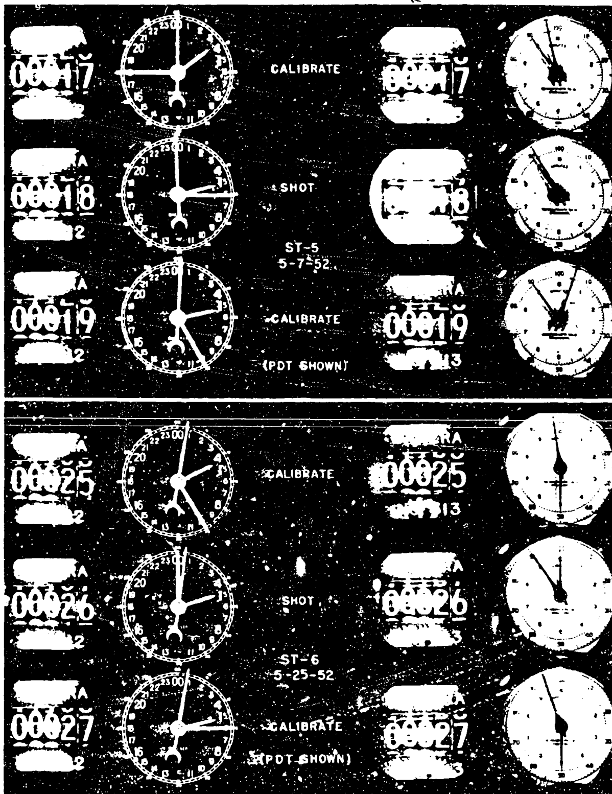
Fig. 2c—Tumbler-Snapper world time readings.
