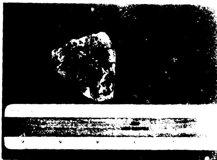
Figure 4. Hardness specimens used in experiments. The diversity of surface on natural specimens required systematic application of the abrasive and microscopic verification that abrasion had occurred (photographs by P. Keene).
