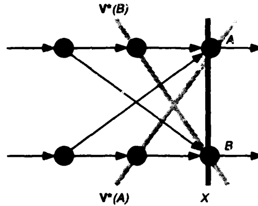
Figure 3.4 Not all timeslices are adjusted vectors. Timeslice X = \{A, B\} equals neither V^*(A) nor V^*(B) . This example disproves the conjecture that Theorem 2.7 might describe all timeslices.
