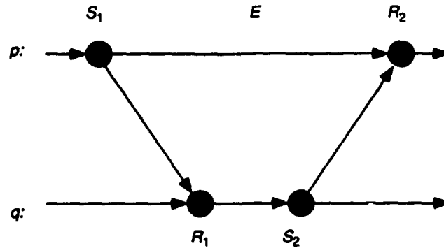
Figure 2.12 Consider the partial order produced by the transitive closure of this event-only graph. Edge E at process p is concurrent with both R_1 and S_2 at process q . However, all nodes at process p either precede R_1 or follow S_2 . Consequently, this graph is not view-complete. As a result, no timeslice can minimally represent a global state containing R_1 or S_2 , since any corresponding process p node will not be concurrent.
