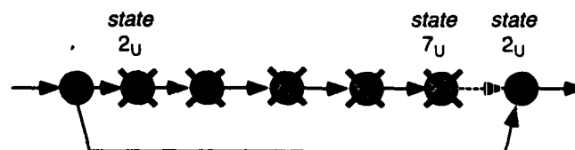
Figure 4.15 Since Theorem 4.1 shows that user precedence implies system precedence, the same drawing can show both USER_PARTIAL_ORDER and SYSTEM_PARTIAL_ORDER information. We use the convention that dashed edges carry precedence in SYSTEM_PARTIAL_ORDER only. This sketch shows that, after rollback, the restored state system-follows the aborted state.
