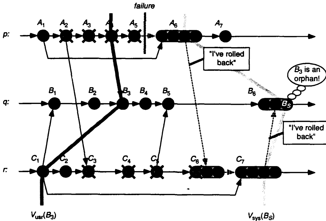
Figure 4.27 DT_ORPHAN_TEST allows accurate orphan elimination. Here, node B_S is the only named system node. At B_S , the system process at q can know that user node B_3 is an orphan, because in the process p timetree, node A_4 (the p entry of V_{usr}(B_3) ) does not precede node A_6 (the USER image of the p entry of V_{sys}(B_S) ).
