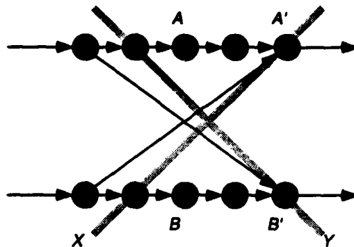
Figure 3.5 Parallax occurs when snapshots appear to be inconsistent. Consider the positions of nodes A and B with respect to timeslices X = V^*(A') and Y = V^*(B') . Both timeslices represent logically simultaneous instants. However, at instant X , A has occurred but B has not, while at instant Y , B has occurred but A has not.
