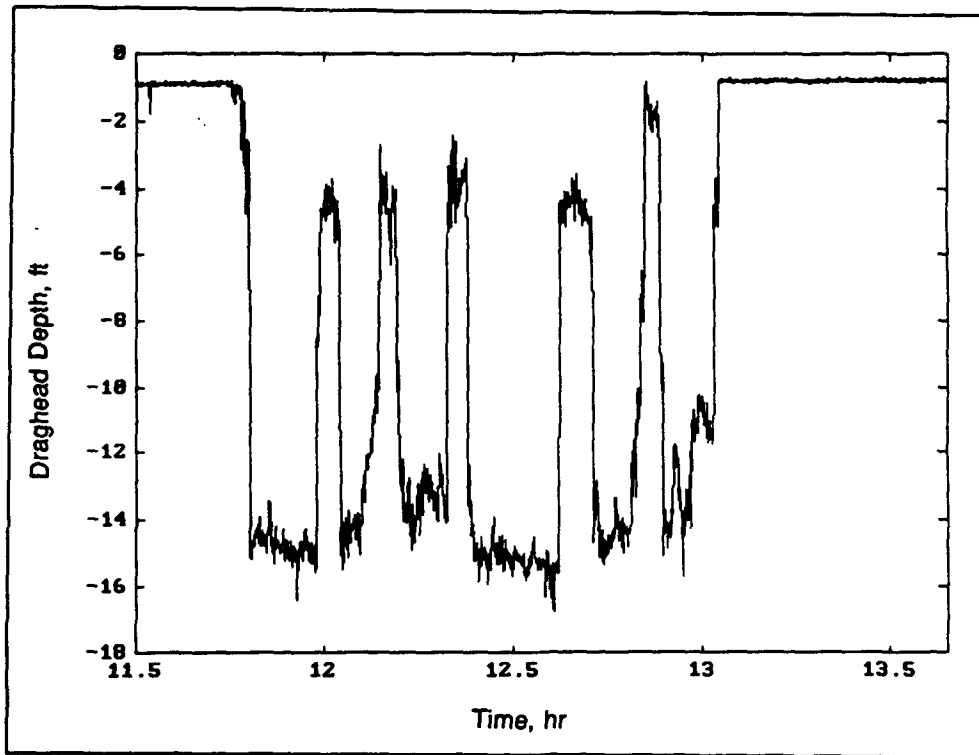
Figure 13. Port draghead depth versus time
