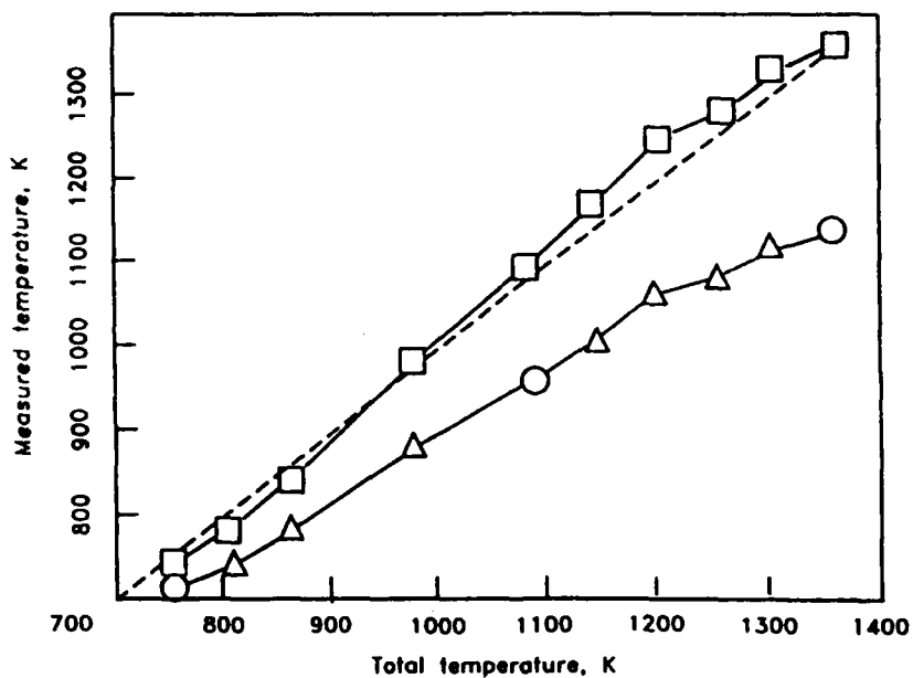
Figure 11: Measured or calculated temperature versus true total temperature from Lagen and Seiner[10]. O - Calibration points, \Delta - measured bead temperature, \square - calculated temperature, ----- ideal calculated temperature.
