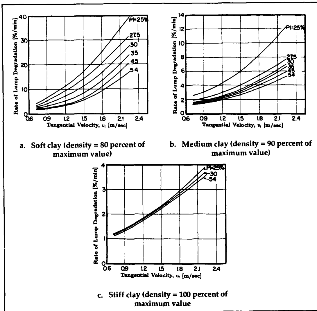
Figure 10. Proposed design charts
