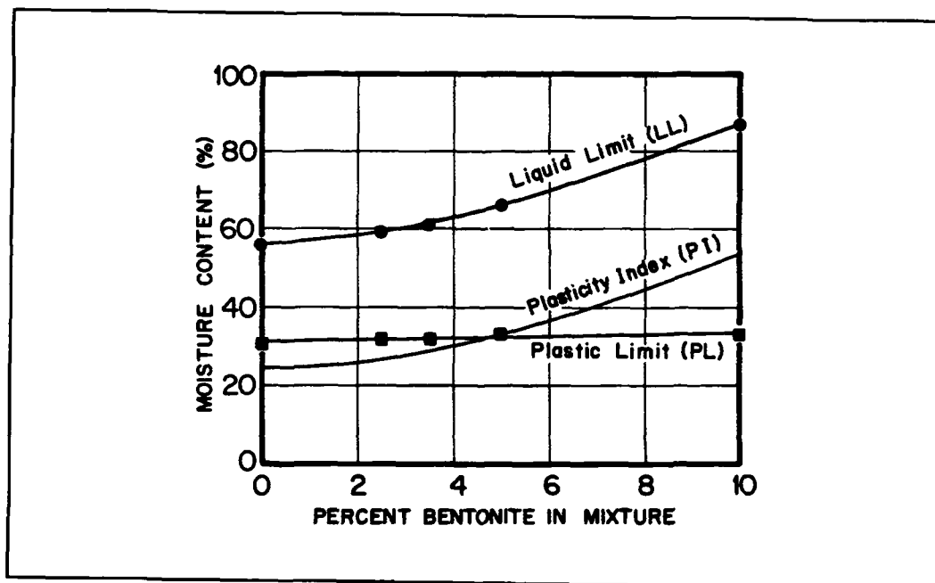
Figure 6. Atterberg limits versus bentonite in mixture
