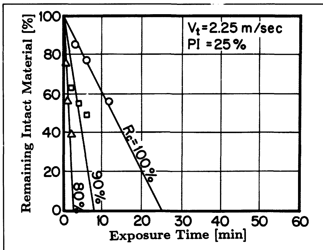
Figure 9. Typical test results (PI = 25 percent and v_t = 2.25 m/sec)
