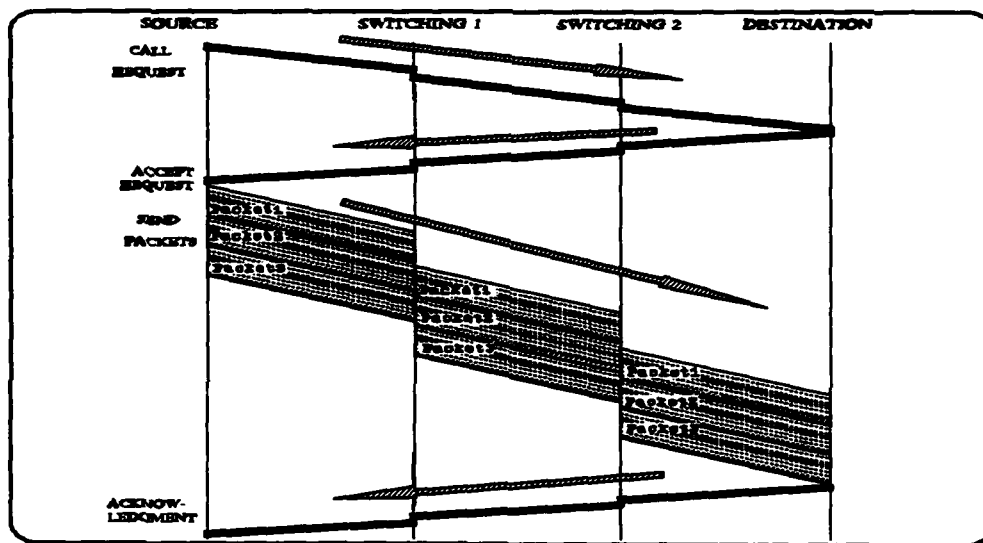
Figure 14. Virtual Circuit
