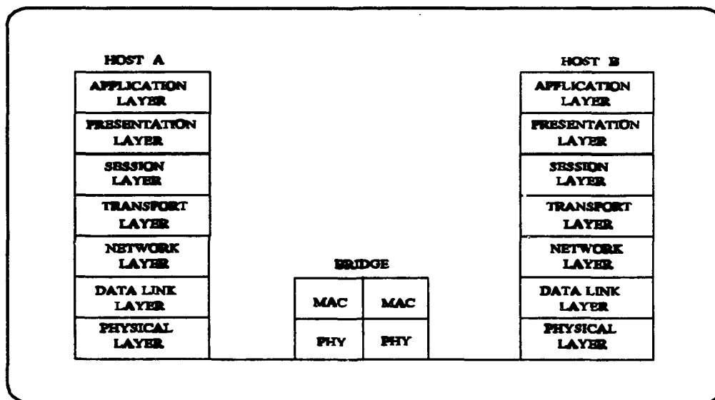
Figure 20. Bridge
