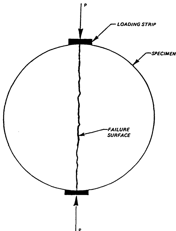
Figure 17. Schematic of Indirect Tensile Test
