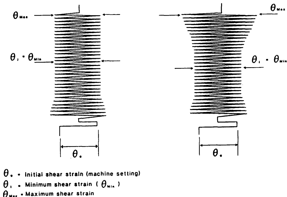
Figure 15. Typical Gyrograph 75
