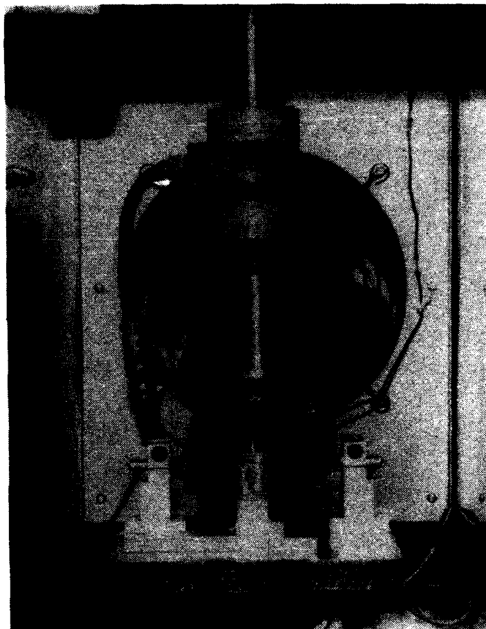
Figure 19. Resilient Modulus Test
