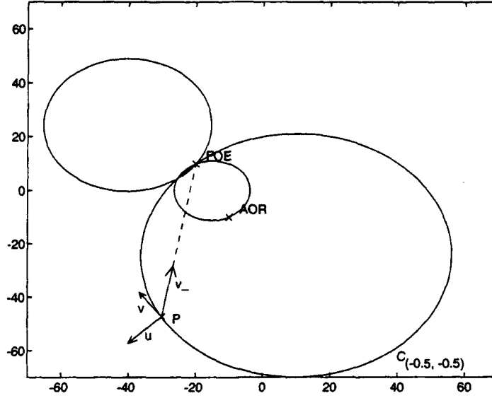
Figure 12: For any point P with motion vector \mathbf{v} on a general \mathbf{u} iso-motion contour the motion vectors \mathbf{v}_- , where \mathbf{v}_- = \mathbf{v} - \mathbf{u} , is parallel to the translational component \mathbf{v} .
