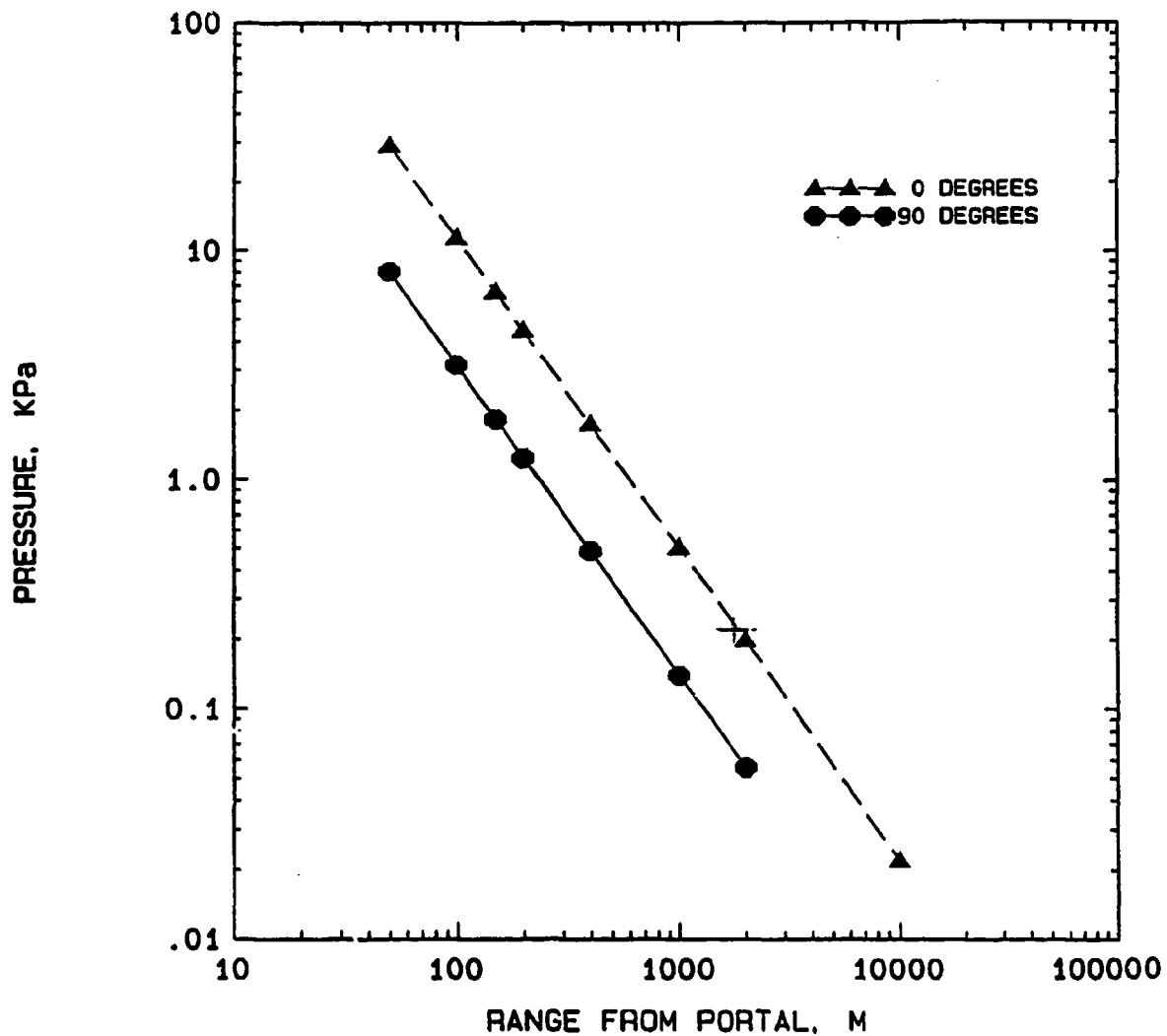
Figure 5. Predicted airblast magnitudes for a 2,800-kg detonation.
