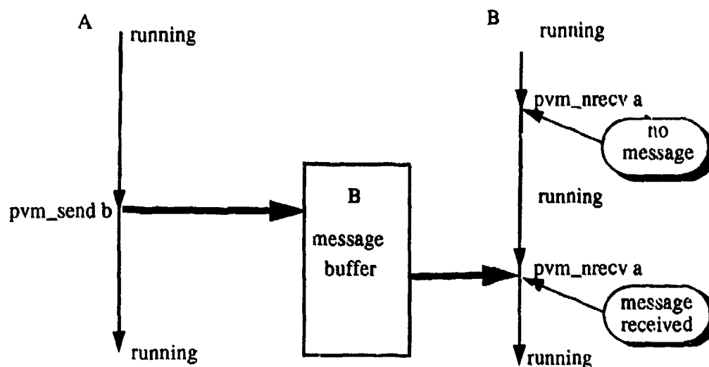
Figure 4.6.2-2 Asynchronous Communications Example: Non-Blocking Receive
