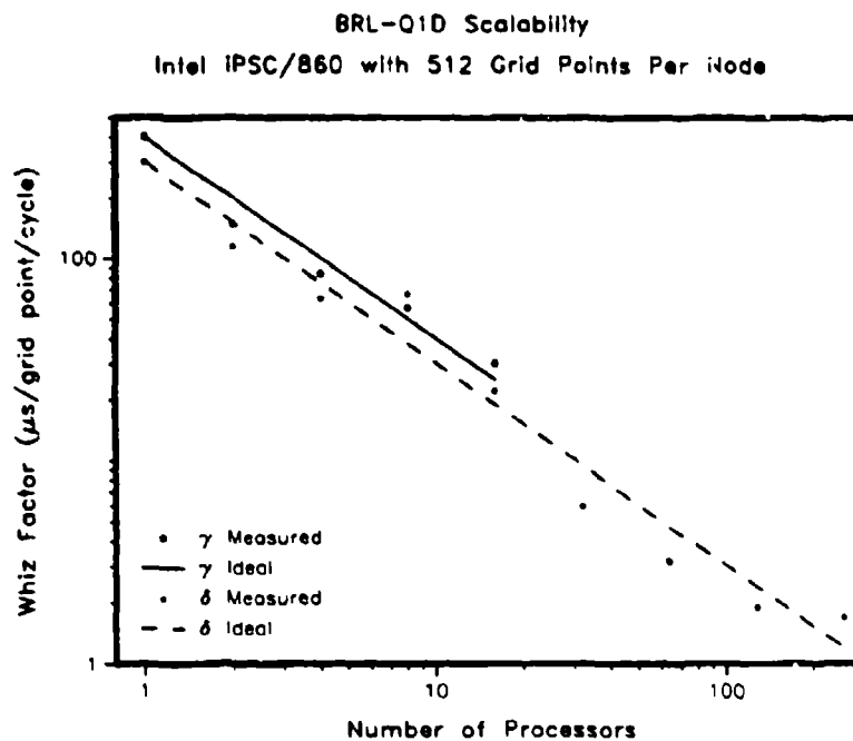
Figure 2. Scalability Using 512 Grid Points / Node
