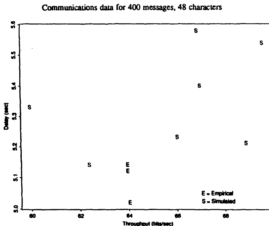
Figure 8. Marginals for a representative data set - throughput vs. delay.
