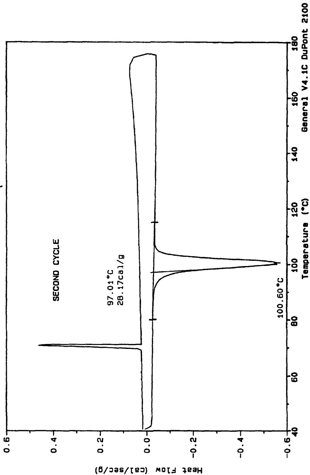
Figure 36. DSC thermogram of 75 mol%/25 mol% TNAZ/2,4-DNI, second cycle through 40-175 °C (5 °C/min)
