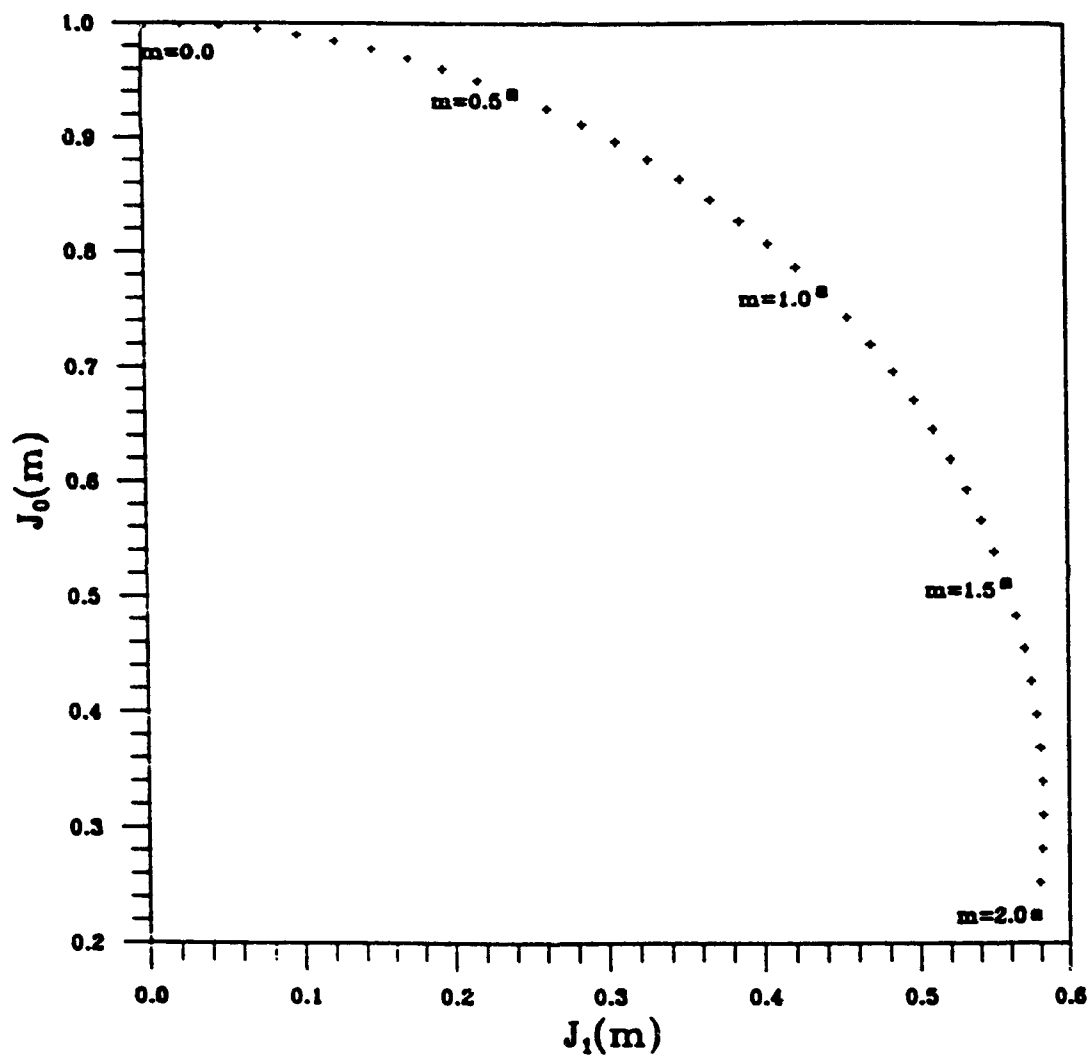
Fig. 2 — Zero-order and first-order Bessel functions as a function of modulation index
