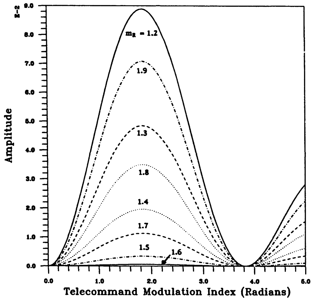
Fig. 23 — Uplink modulation loss for squarewave ranging vs telecommand as a function of modulation index for ranging modulation index from 1.2 to 1.9
