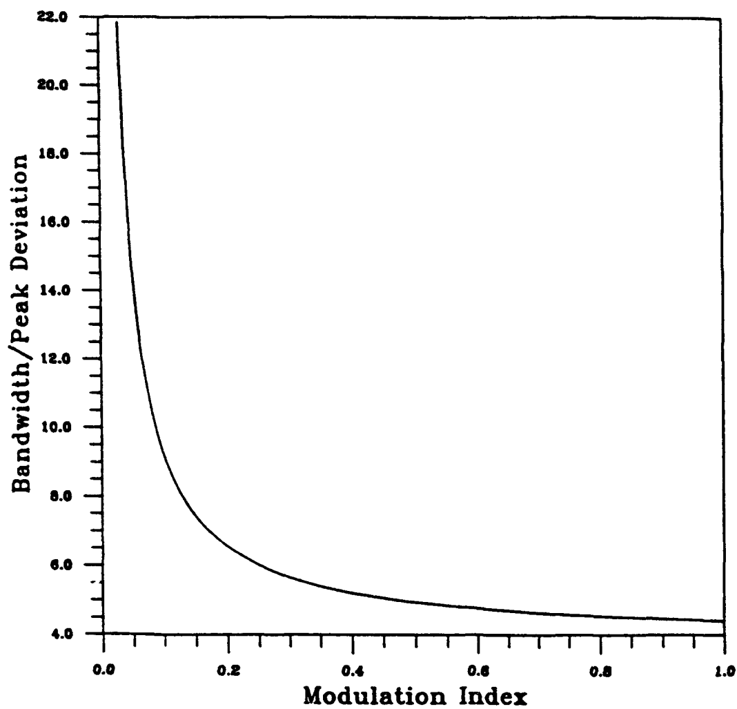
Fig. 6 — Necessary bandwidth plot for frequency-shift-keying as a function of modulation index (range 0.0 to 1.0)
