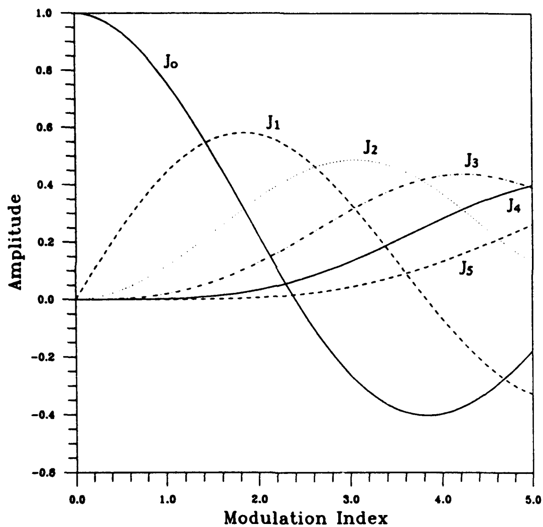
Fig. 1— Plots of first six Bessel functions vs modulation index
