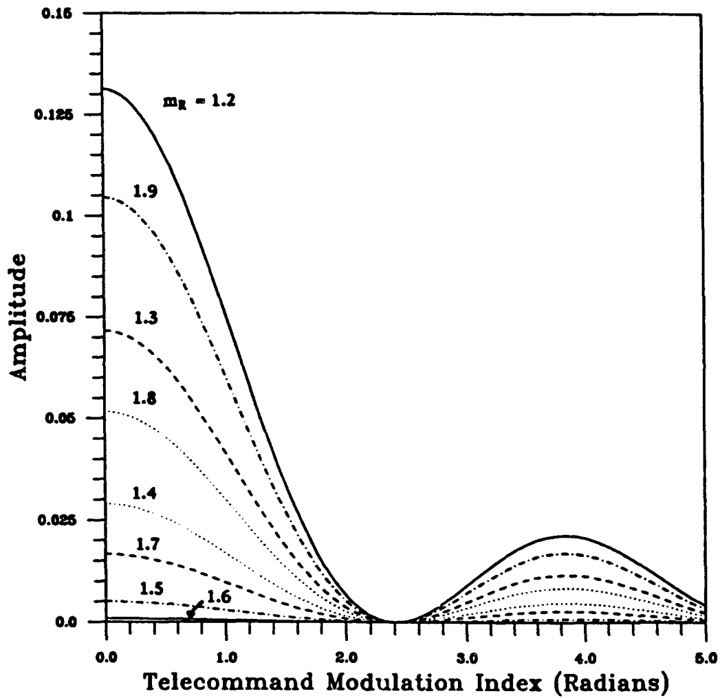
Fig. 20 — Uplink modulation loss for squarewave ranging vs carrier as a function of modulation index for ranging modulation index from 1.2 to 1.9
