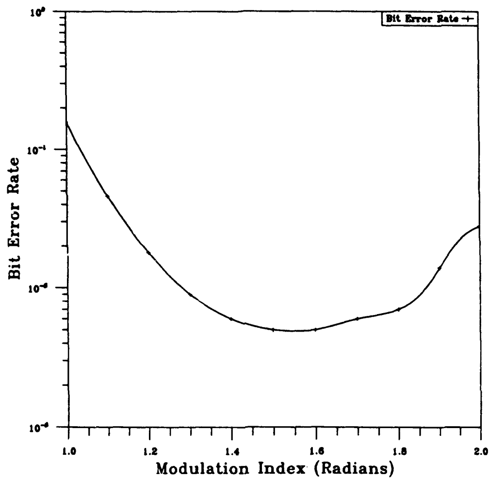
Fig. 15 — Bit error probability for DSPSE asteroid encounter omni antenna for DSN 34 m ground as a function of modulation index
