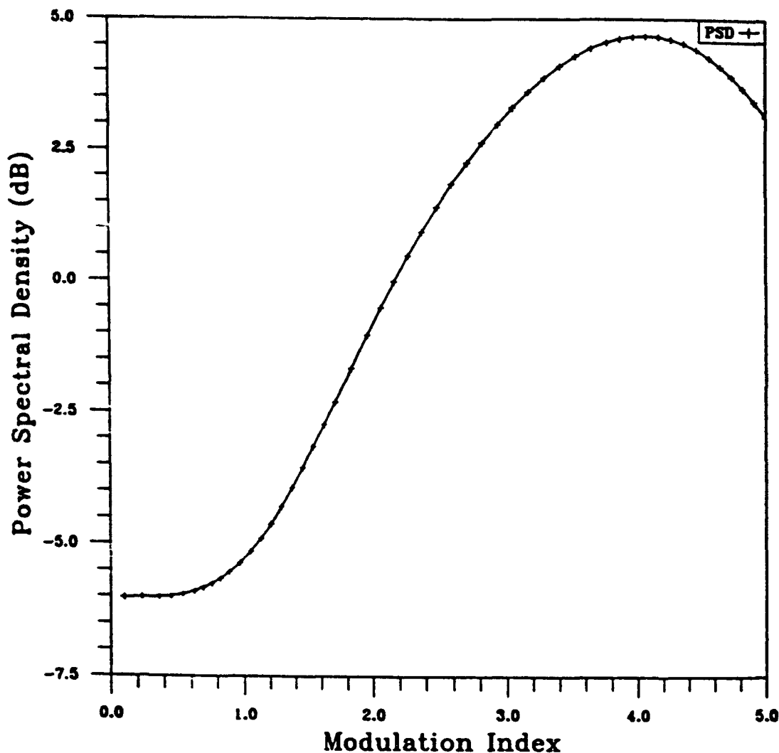
Fig. 5 — Power spectral density function of frequency-shift-keying as a function of modulation index
