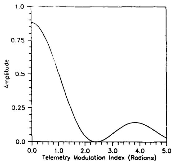
Fig. 27 — Downlink modulation loss for sinusoid ranging vs carrier as a function of modulation index (range of 0.1 to 5.0)
