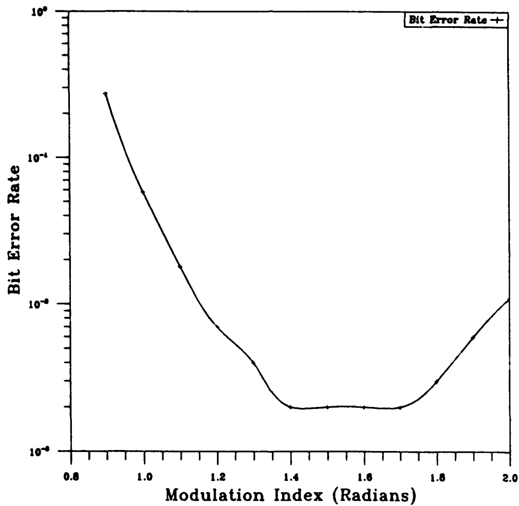
Fig. 16 — Bit error probability for DSPSE asteroid encounter high-gain antenna for DSN 34 m ground as a function of modulation
