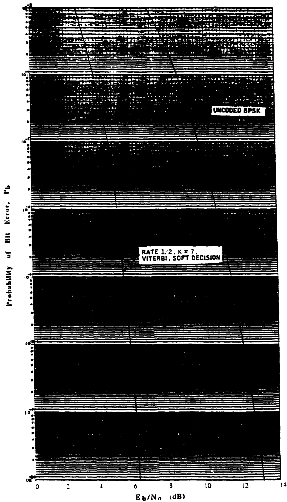
Fig. 11 — Bit error probability vs bit energy-to-noise power spectral density for Viterbi coded and uncoded BPSK
