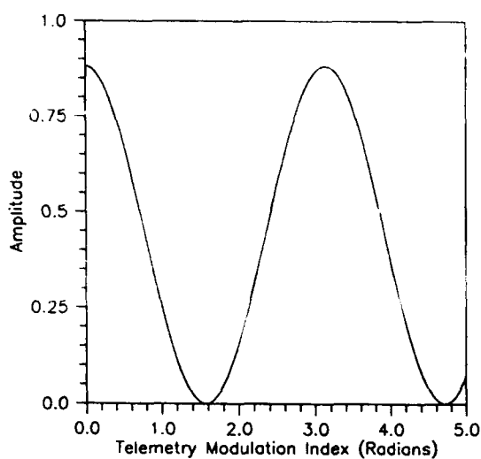
Fig. 26 — Downlink modulation loss for square-wave ranging vs carrier as a function of modulation index (range of 0.0 to 5.0)
