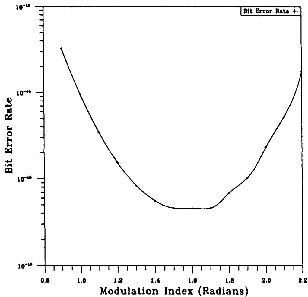
Fig. 12 — Bit error probability for DSPSE lunar mission high-gain antenna for 26 m ground as a function of modulation index
