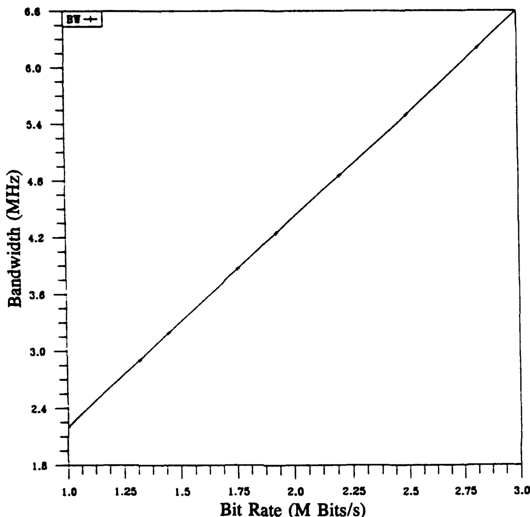
Fig. 10—Necessary bandwidth plot for sinusoidal frequency-shift-keying
