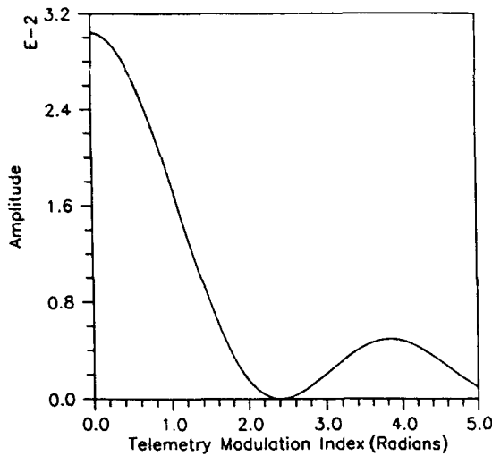
Fig. 30 — Downlink modulation loss for squarewave ranging vs ranging as a function of modulation index (range of 0.0 to 5.0)
