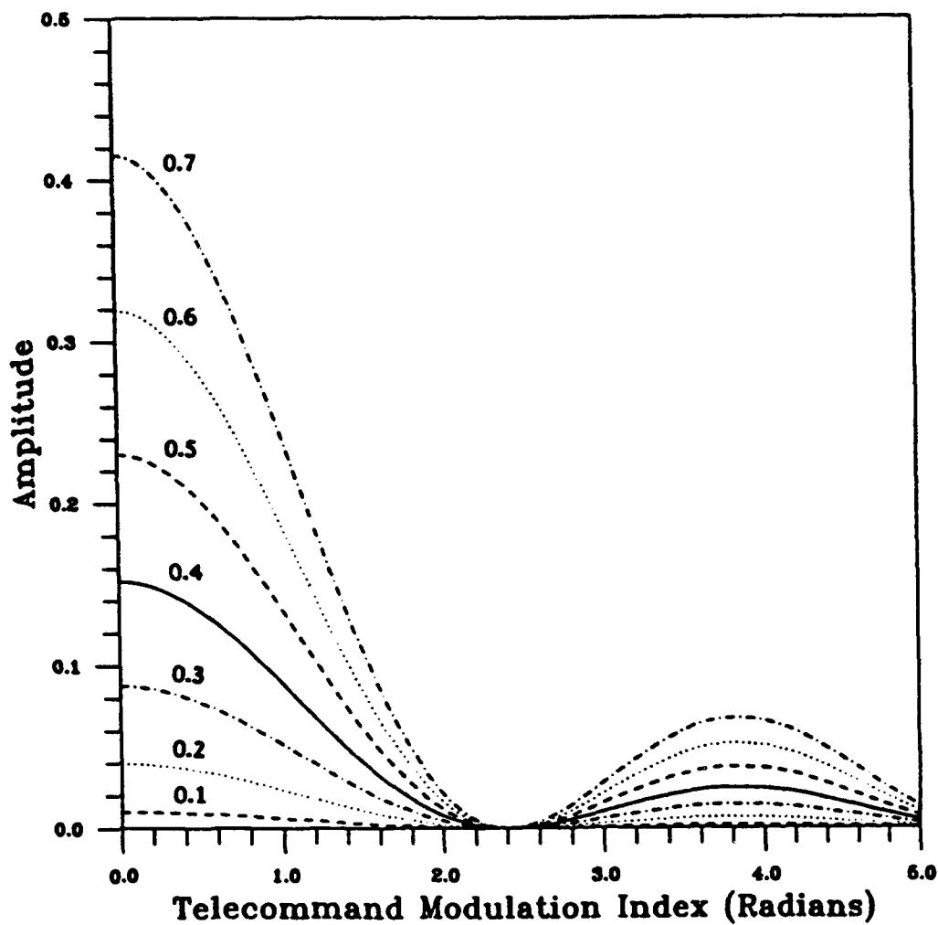
Fig. 24— Uplink modulation loss for squarewave ranging vs ranging as a function of modulation index for ranging modulation index from 0.0 to 0.7
