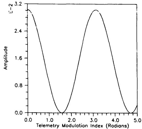
Fig. 31 — Downlink modulation loss for sinusoid ranging vs ranging as a function of modulation index (range of 0.0 to 5.0)
