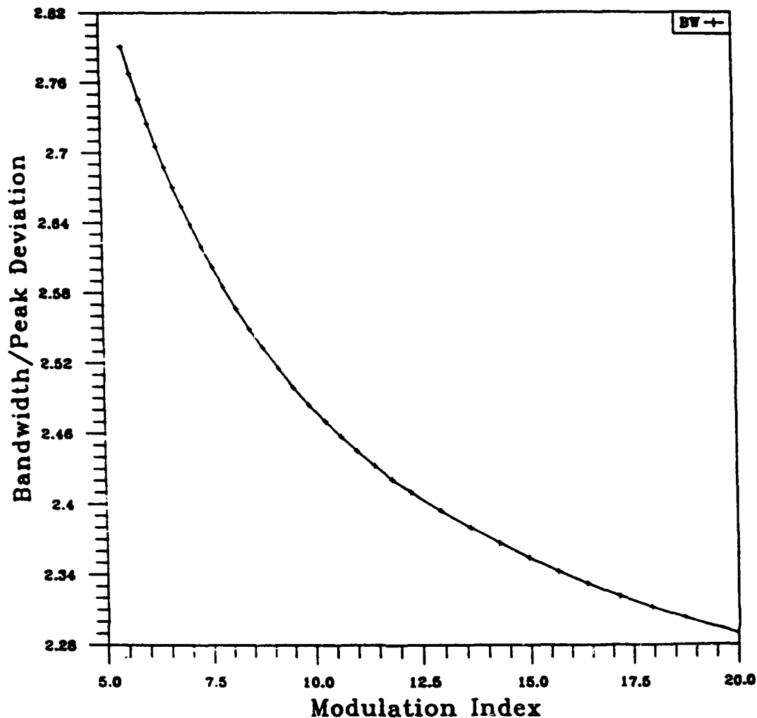
Fig. 8 — Necessary bandwidth plot for frequency-shift-keying as a function of modulation index (range 5.0 to 20.0)
