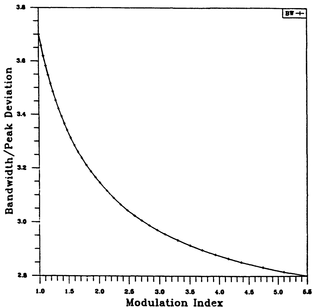
Fig. 7 — Necessary bandwidth plot for frequency-shift-keying as a function of modulation index (range 1.0 to 5.5)
