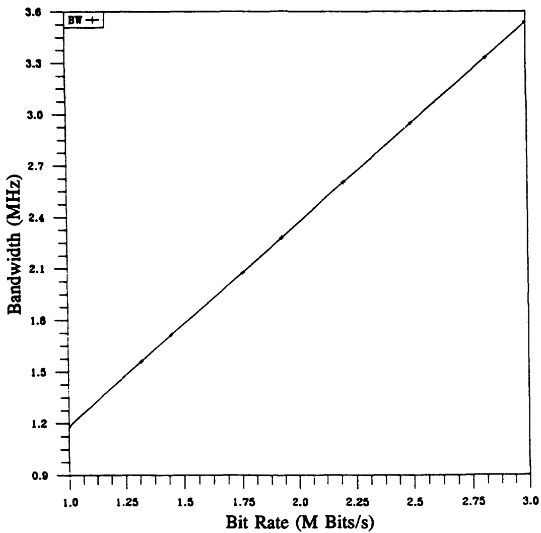
Fig. 9 — Necessary bandwidth plot for minimum-shift-keying
