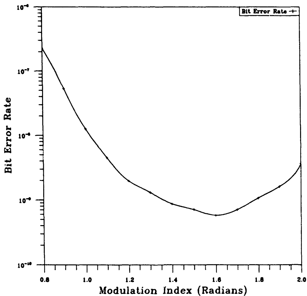
Fig. 18 — Bit error probability for DSPSE asteroid encounter high-gain antenna for DSN 70 m ground as a function of modulation index
