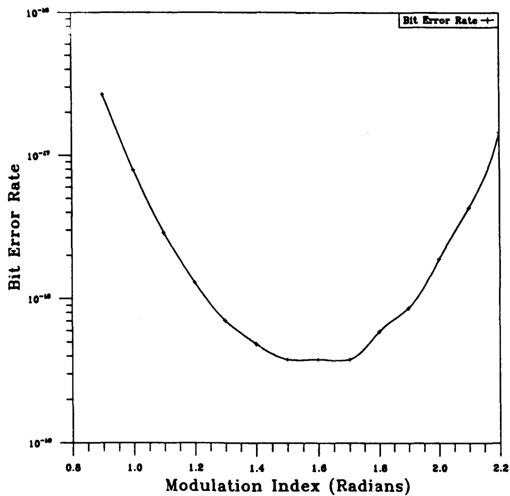
Fig. 13 — Bit error probability for DSPSE mission omni antenna for 30 m ground as a function of modulation index
