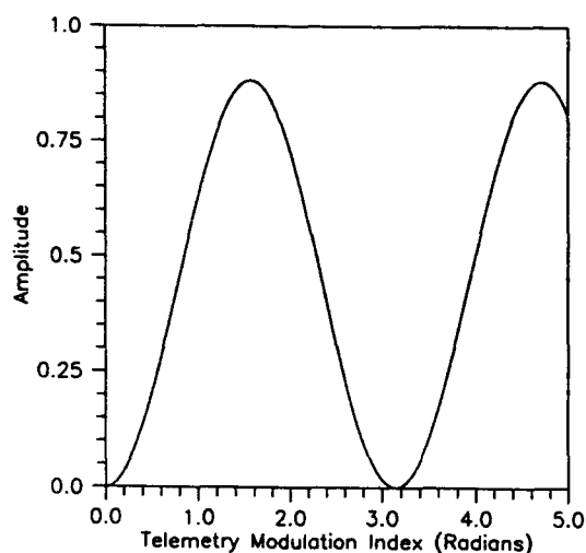
Fig. 28 — Downlink modulation loss for squarewave ranging vs telemetry as a function of modulation index (range of 0.0 to 5.0)
