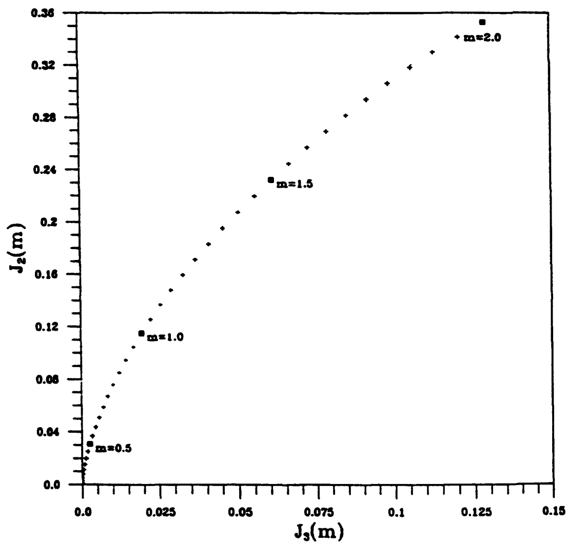
Fig. 3 — Second-order and third-order Bessel functions as a function of modulation index
