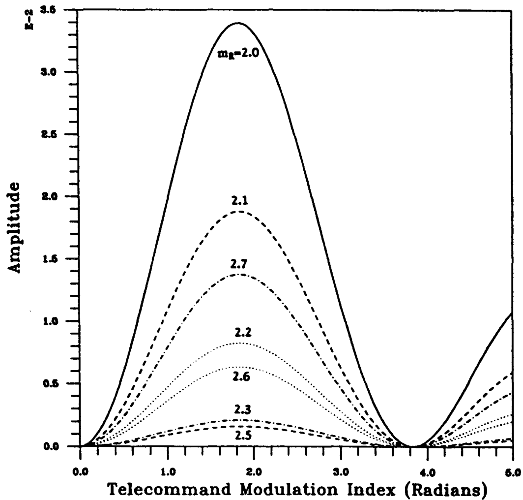
Fig. 22 — Uplink modulation loss for sinusoid ranging vs telecommand as a function of modulation index for ranging modulation index from 2.0 to 2.7
