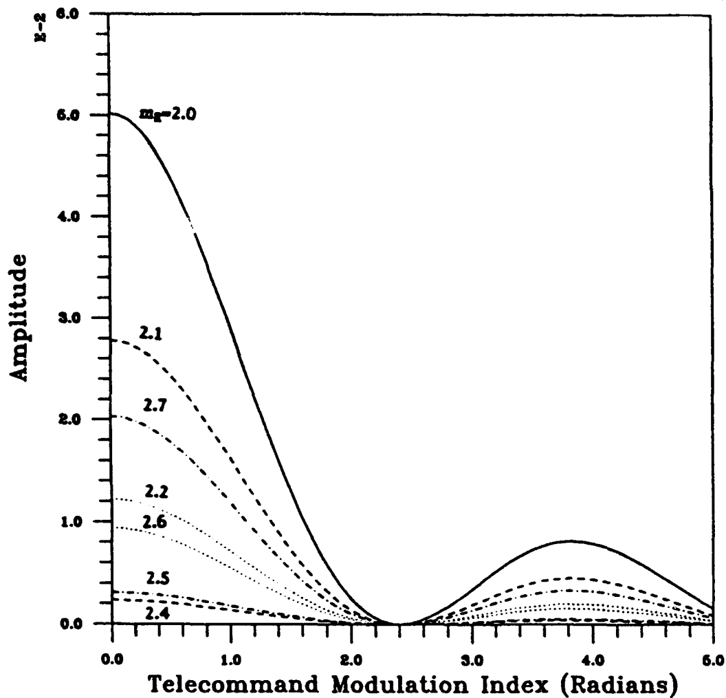
Fig. 25 — Uplink modulation loss for sinusoid ranging vs carrier as a function of modulation index for ranging modulation index from 2.0 to 2.7
