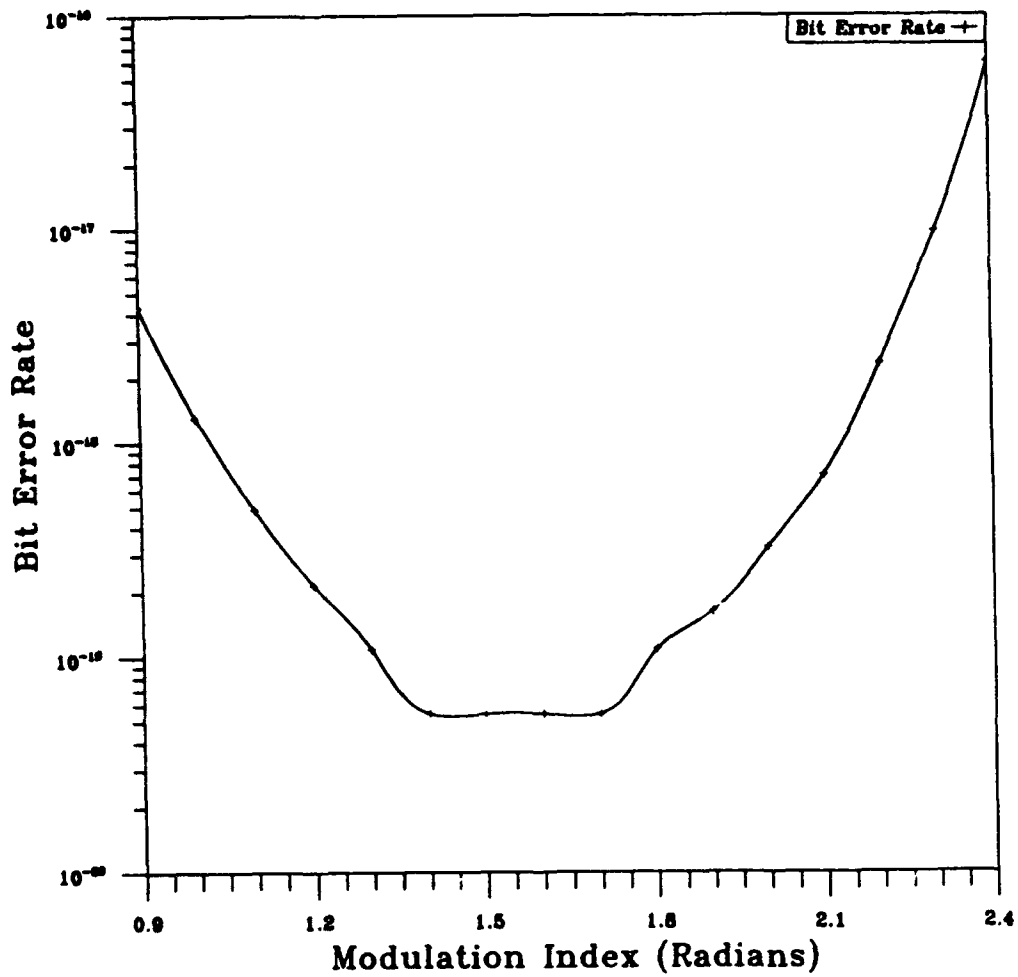
Fig. 14 — Bit error probability for DSPSE lunar mission high-gain antenna for 30 m ground as a function of modulation index
