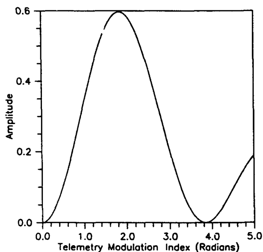
Fig. 29 — Downlink modulation loss for sinusoid ranging vs telemetry as a function of modulation index (range of 0.0 to 5.0)
