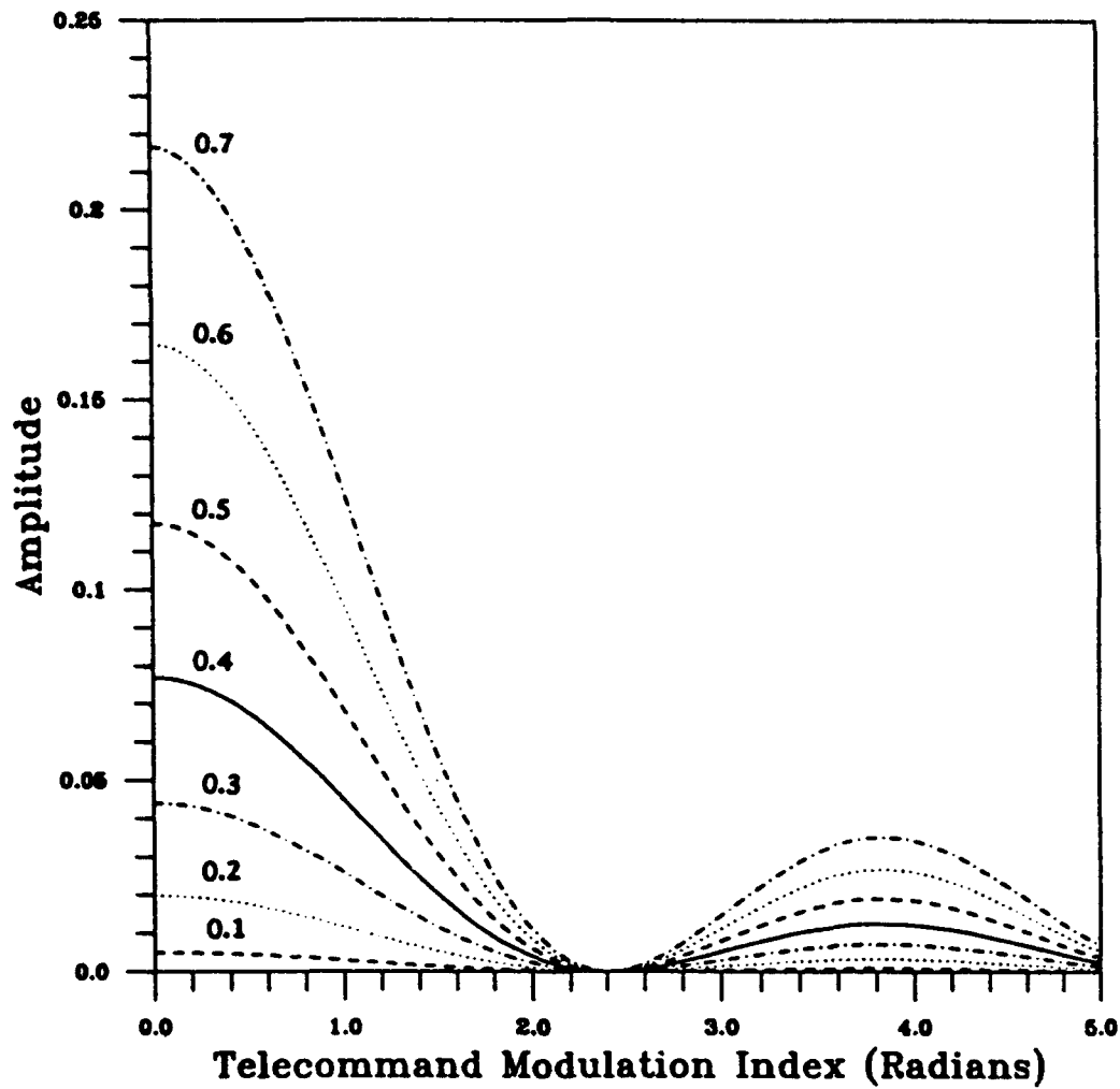
Fig. 21 — Uplink modulation loss for sinusoid ranging vs ranging as a function of modulation index for ranging modulation index from 0.0 to 0.7
