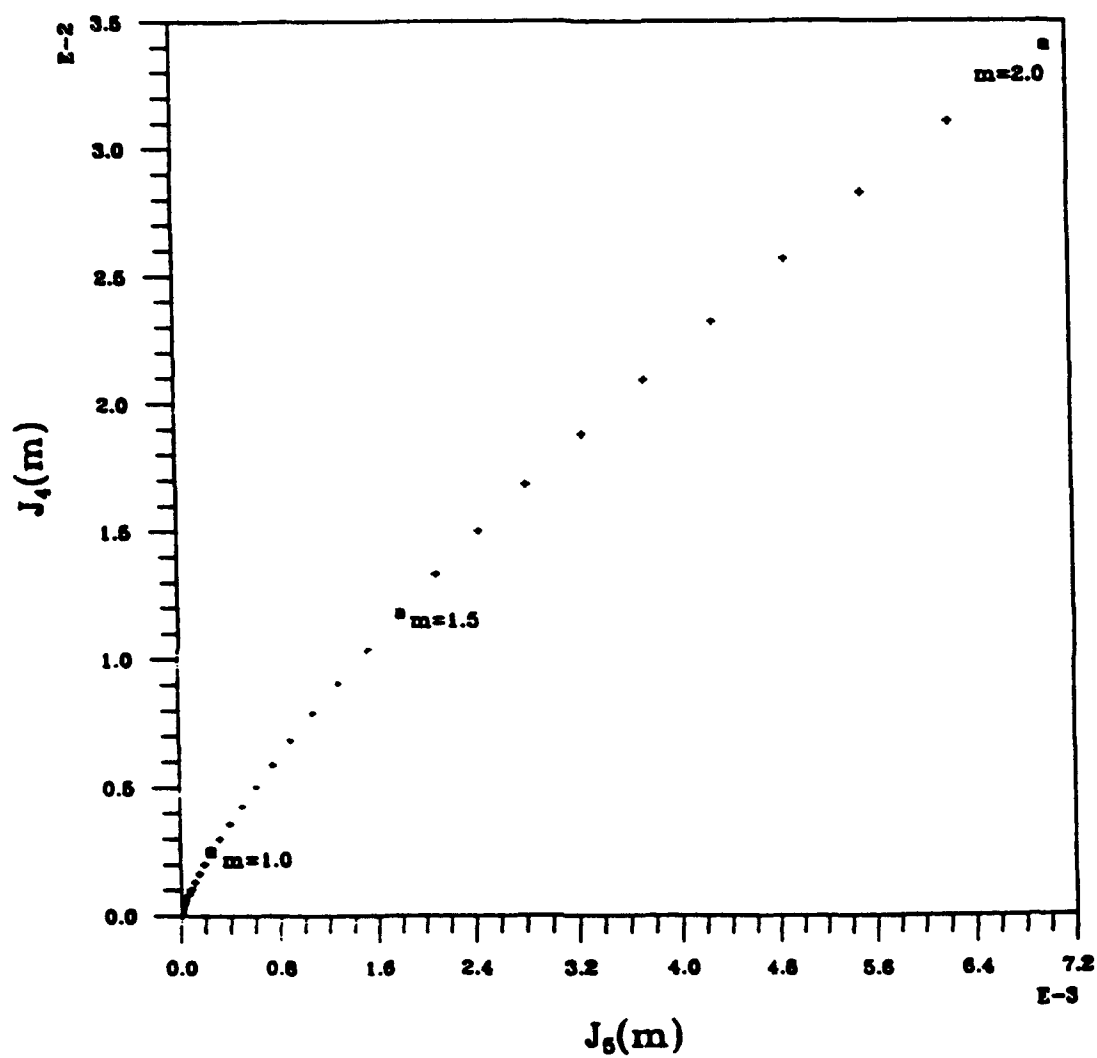
Fig. 4 — Fourth-order and fifth-order Bessel functions as a function of modulation index
