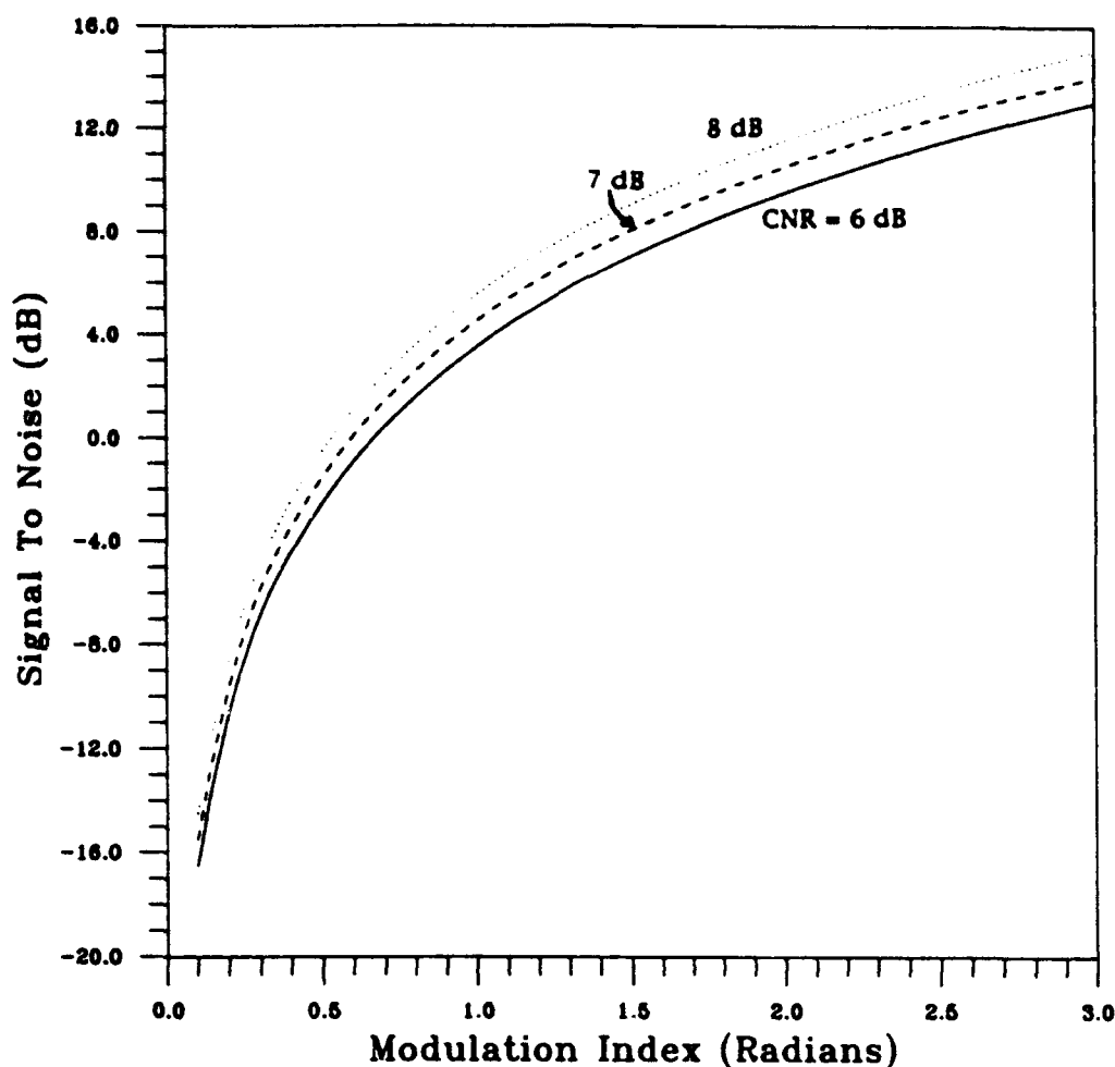
Fig. 32 — Radio frequency (RF) signal-to-noise ratio as a function of modulation index (range of 0.0 to 3.0)
