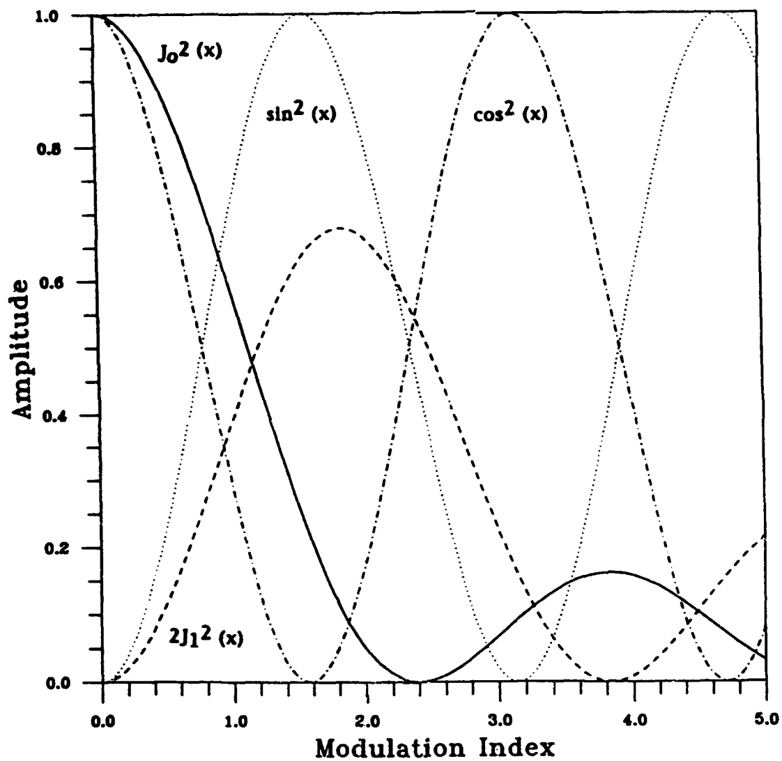
Fig. 19 — Squares of sinusoid and Bessel functions of zero- and first-order as a function of modulation index (range of 0.0 to 5.0)
