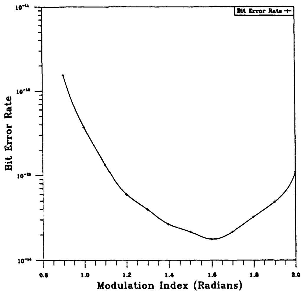
Fig. 17 — Bit error probability for DSPSE lunar mission omni antenna for DSN 70 m ground as a function of modulation index
