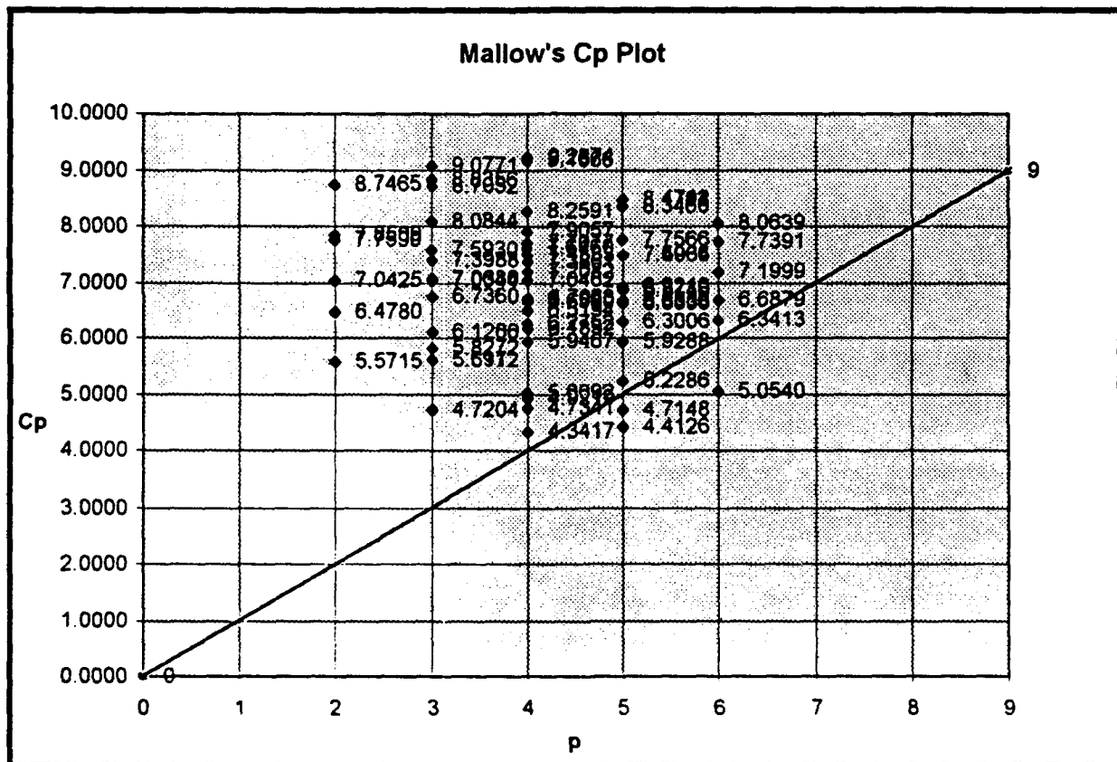
Figure 1. Mallow's Cp Plot
