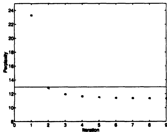
Figure 4: 2.5M corpus
