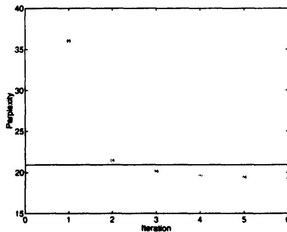
Figure 5: 25M corpus
