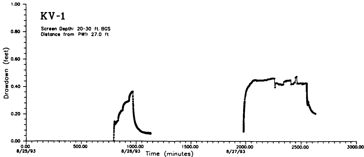
Figure 4-4. Pumping Test Hydrograph for Wells KV-4A, KV-3, and KV-1
