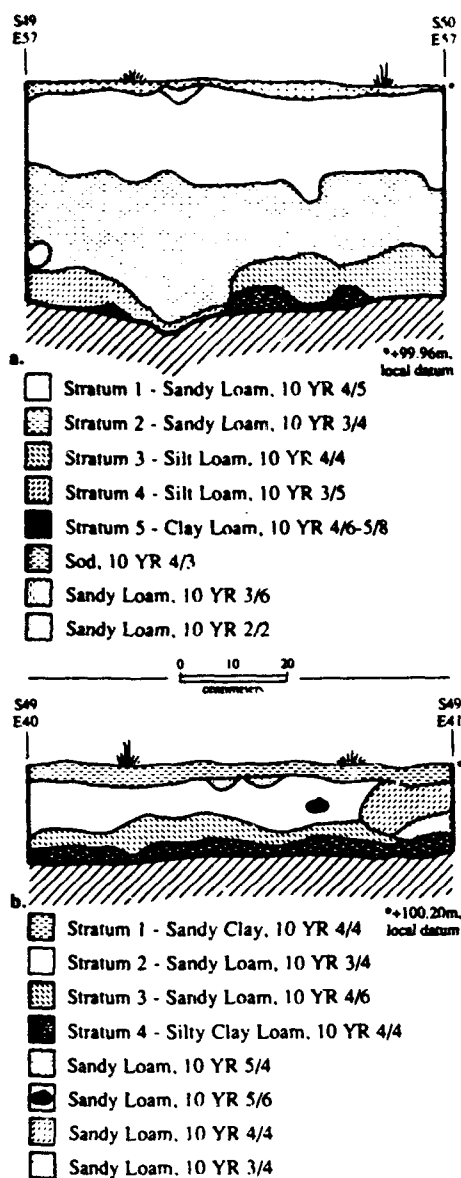
Figure 4.42a Profile of east wall of TP 1, 41DN384; 4.42b Profile of north wall of TP 3, 41DN384.
