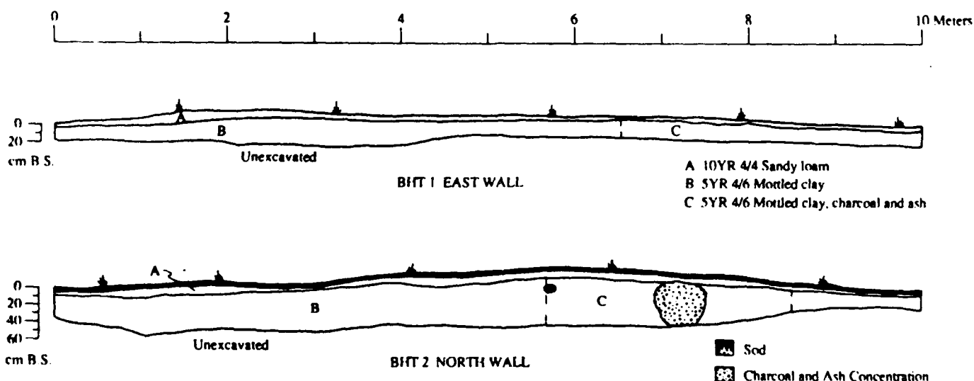
Figure 8.40 Profiles of BHTs 1 and 2 at 41DN429.
